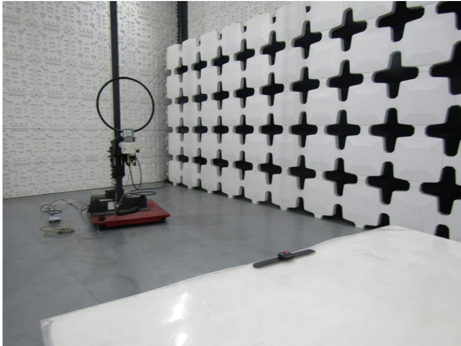
Emission (Below 1GHz)
