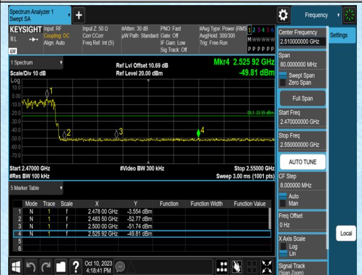
3DH5-Ant1-Hop_2480
