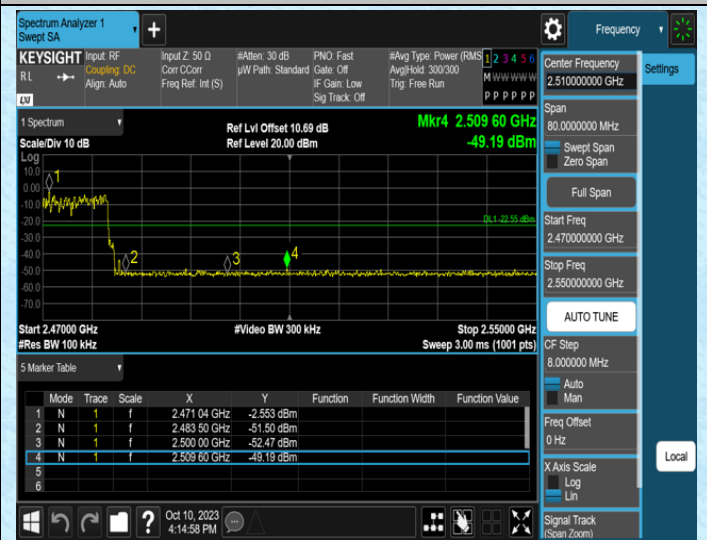
2DH5-Ant1-Hop_2480
