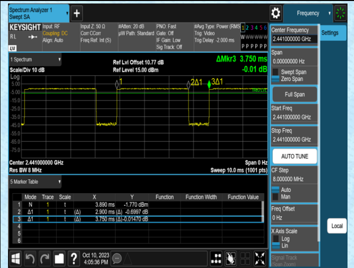
NTNV-3DH5-Ant1-2441
