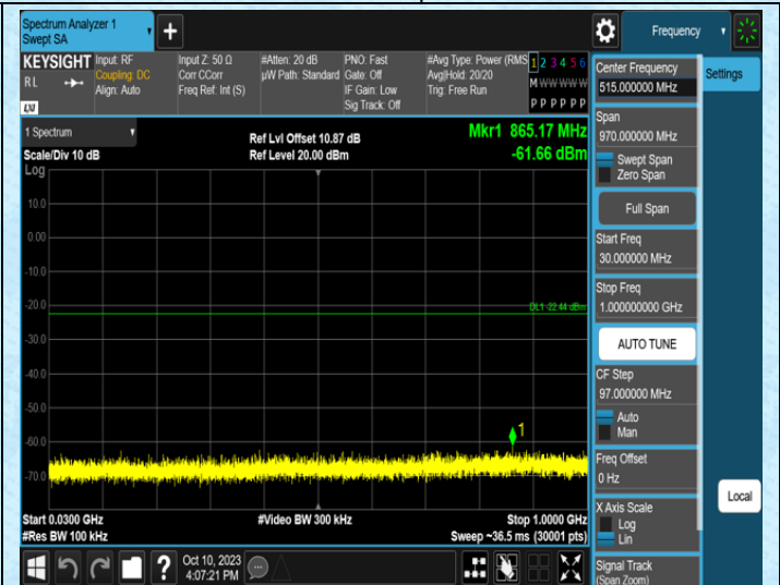
3DH5-Ant1-2480-30~1000
