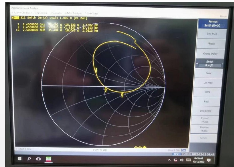
Smith-Chart
