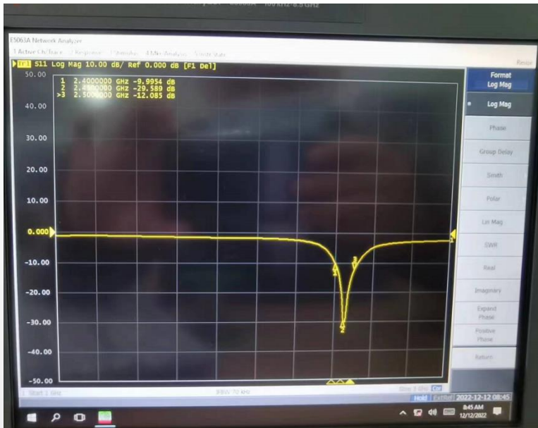
Return loss
