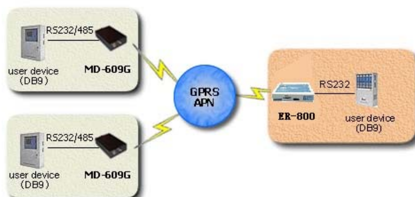
Figure Appendix 3-1: Embedded data center and APN network solution
