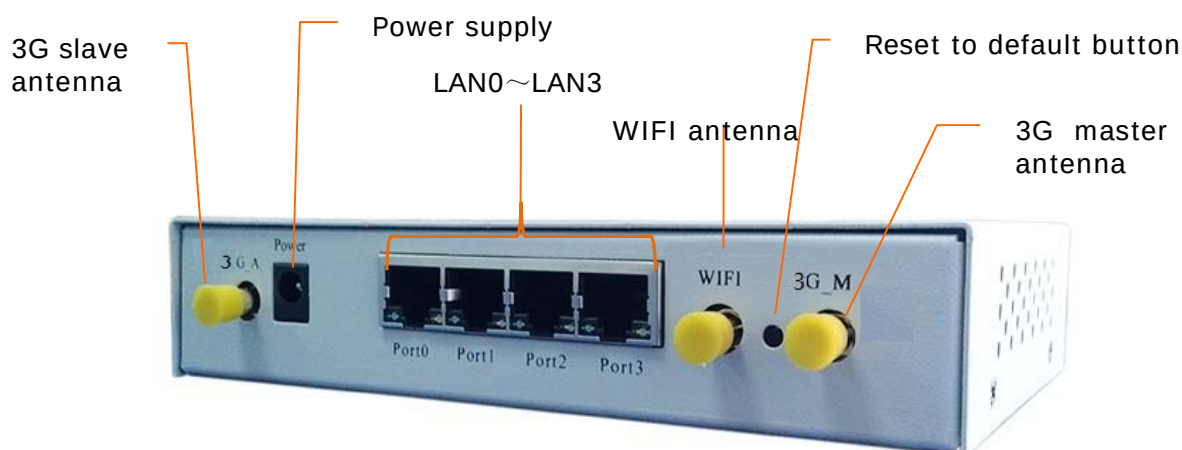
Figure 1-2: ER-800 side view 1
