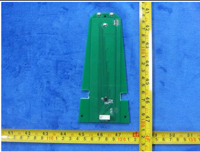
Sma Board 1 - Front View
