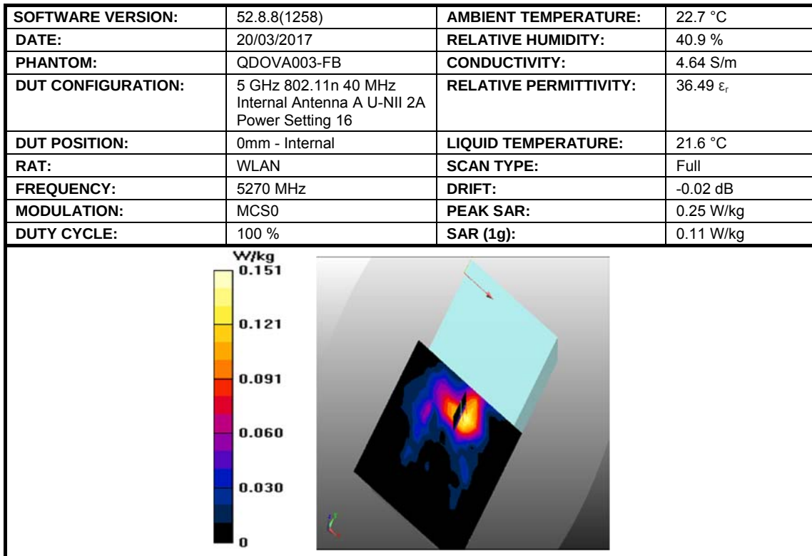
Figure 6: SAR Head Testing Results for the DAQRI Smart Helmet at 5270 MHz.
