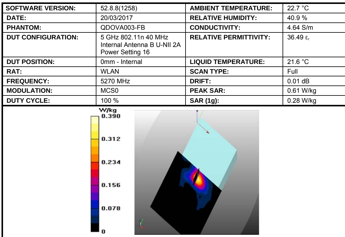
Figure 7: SAR Head Testing Results for the DAQRI Smart Helmet at 5270 MHz.
