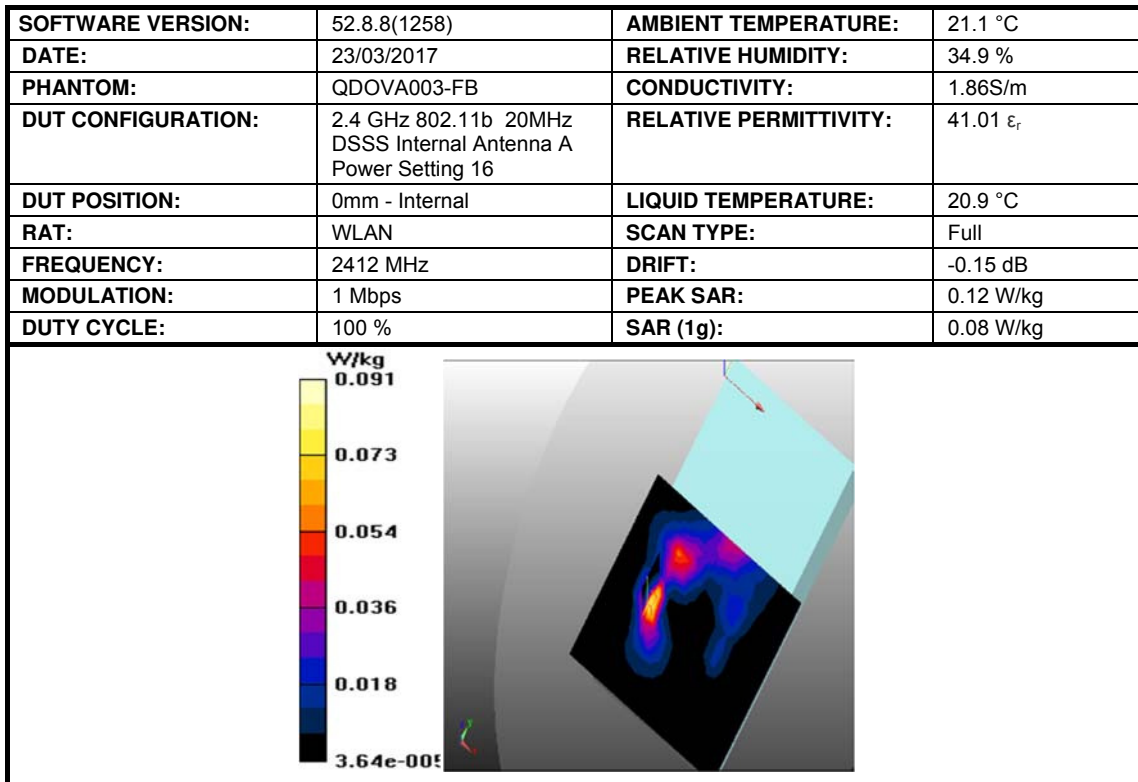
Figure 2: SAR Head Testing Results for the DAQRI Smart Helmet at 2412 MHz.
