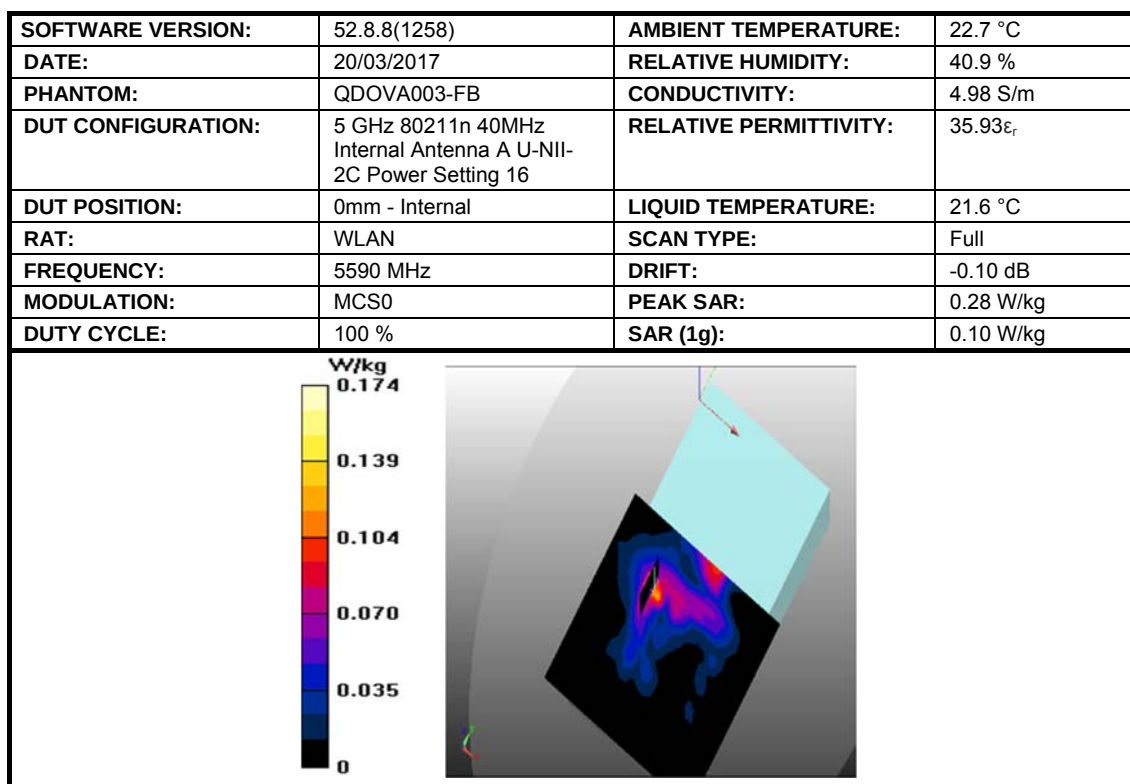
Figure 10: SAR Head Testing Results for the DAQRI Smart Helmet at 5590 MHz.
