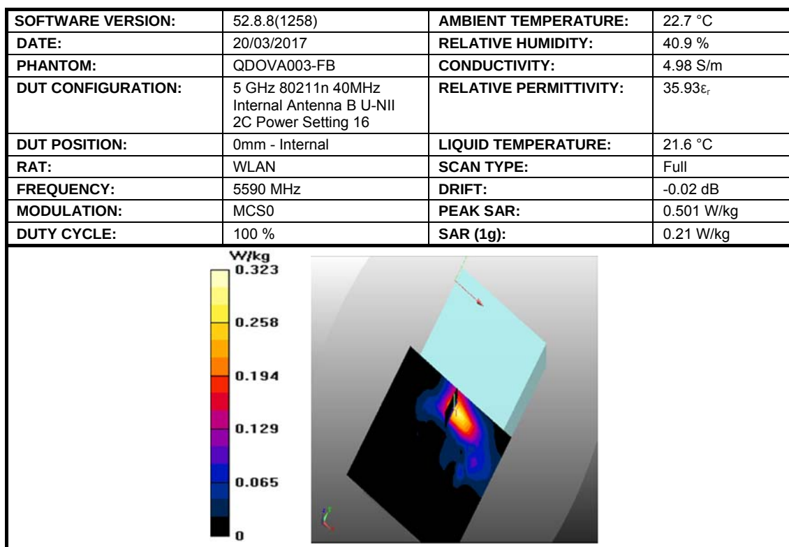
Figure 11: SAR Head Testing Results for the DAQRI Smart Helmet at 5590 MHz.
