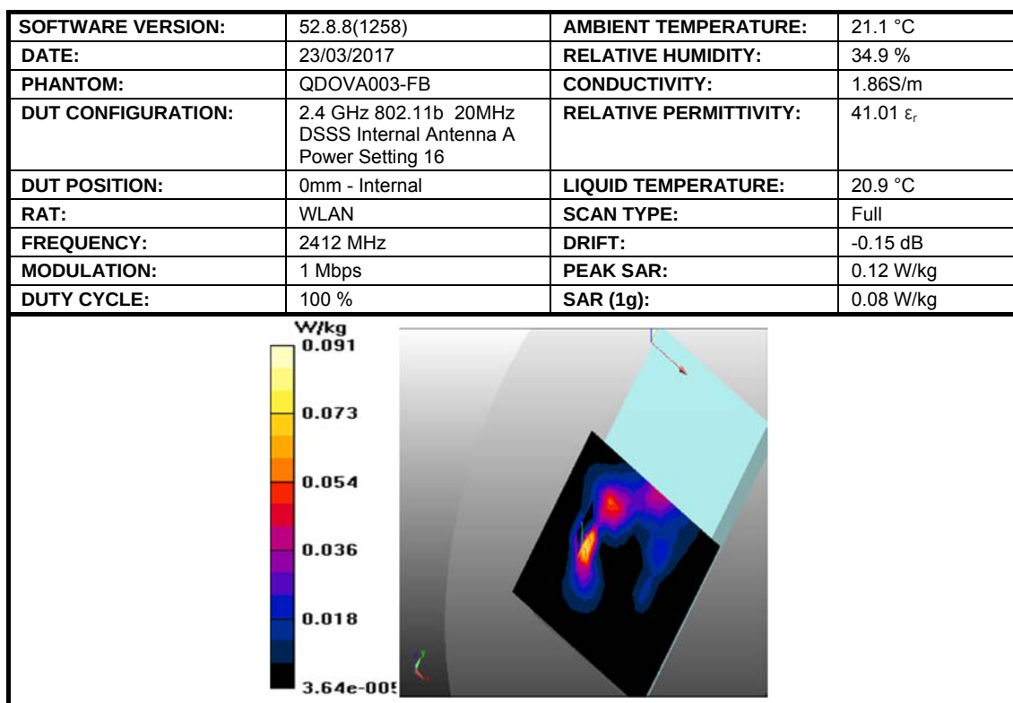
Figure 2: SAR Head Testing Results for the DAQRI Smart Helmet at 2412 MHz.
