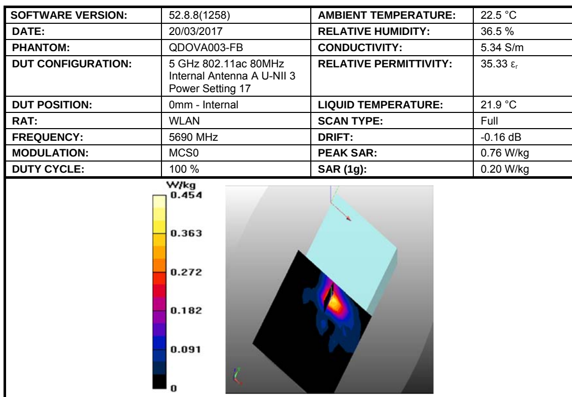
Figure 14: SAR Head Testing Results for the DAQRI Smart Helmet at 5690 MHz.
