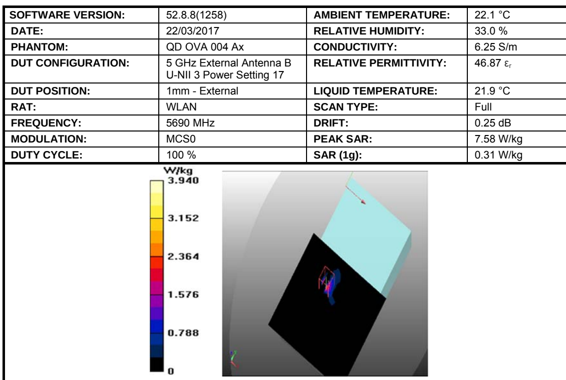
Figure 16: SAR Body-Extremity Testing Results for the DAQRI Smart Helmet at 5690 MHz.
