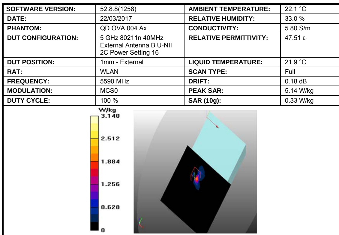
Figure 13: SAR Body-Extremity Testing Results for the DAQRI Smart Helmet at 5590 MHz.
