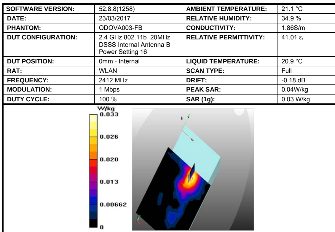
Figure 3: SAR Head Testing Results for the DAQRI Smart Helmet at 2412 MHz.
