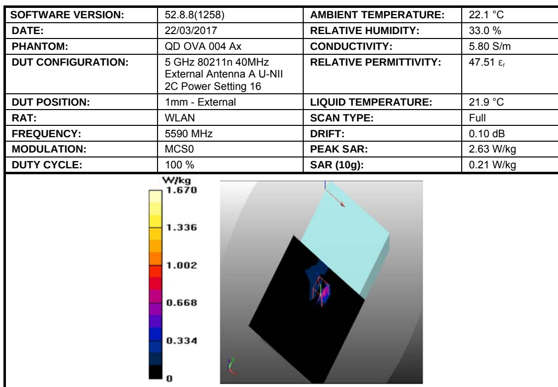
Figure 12: SAR Body-Extremity Testing Results for the DAQRI Smart Helmet at 5590 MHz.
