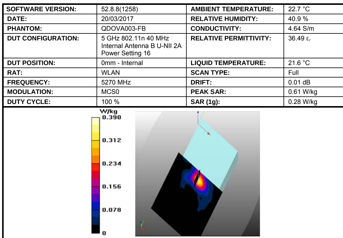
Figure 7: SAR Head Testing Results for the DAQRI Smart Helmet at 5270 MHz.
