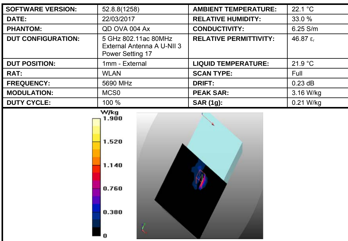
Figure 16: SAR Body-Extremity Testing Results for the DAQRI Smart Helmet at 5690 MHz.
