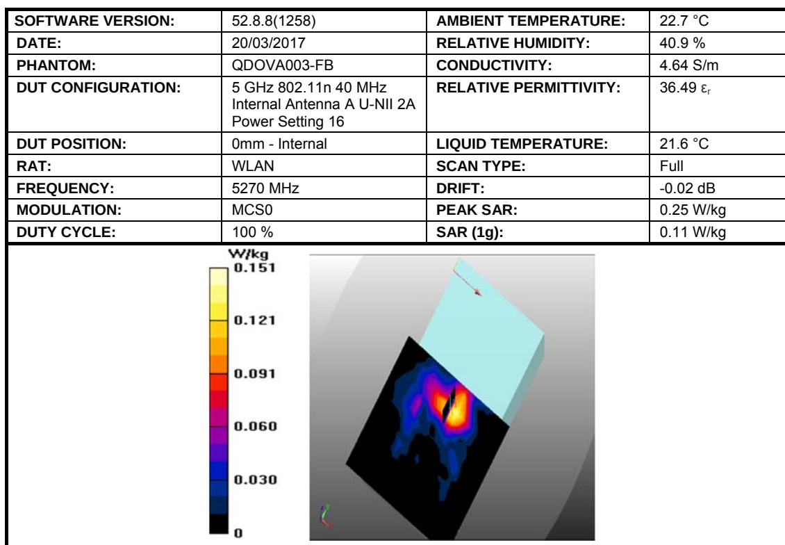
Figure 6: SAR Head Testing Results for the DAQRI Smart Helmet at 5270 MHz.
