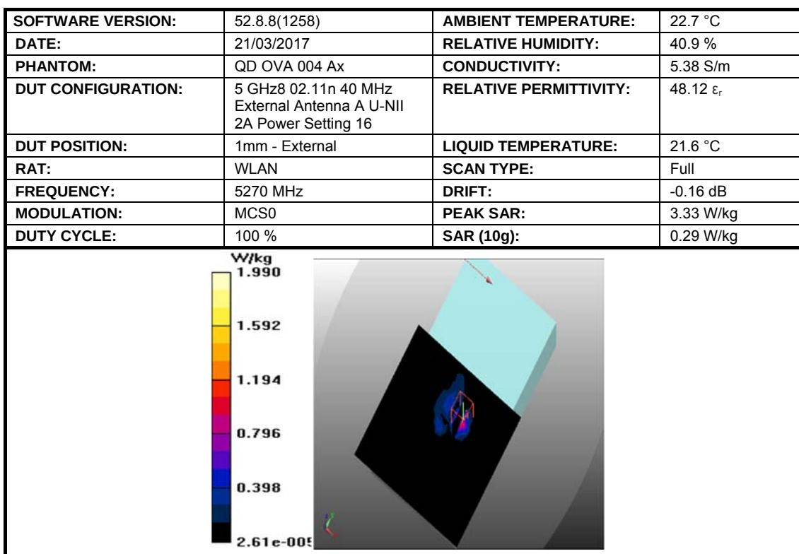
Figure 8: SAR Body-Extremity Testing Results for the DAQRI Smart Helmet at 5270 MHz.
