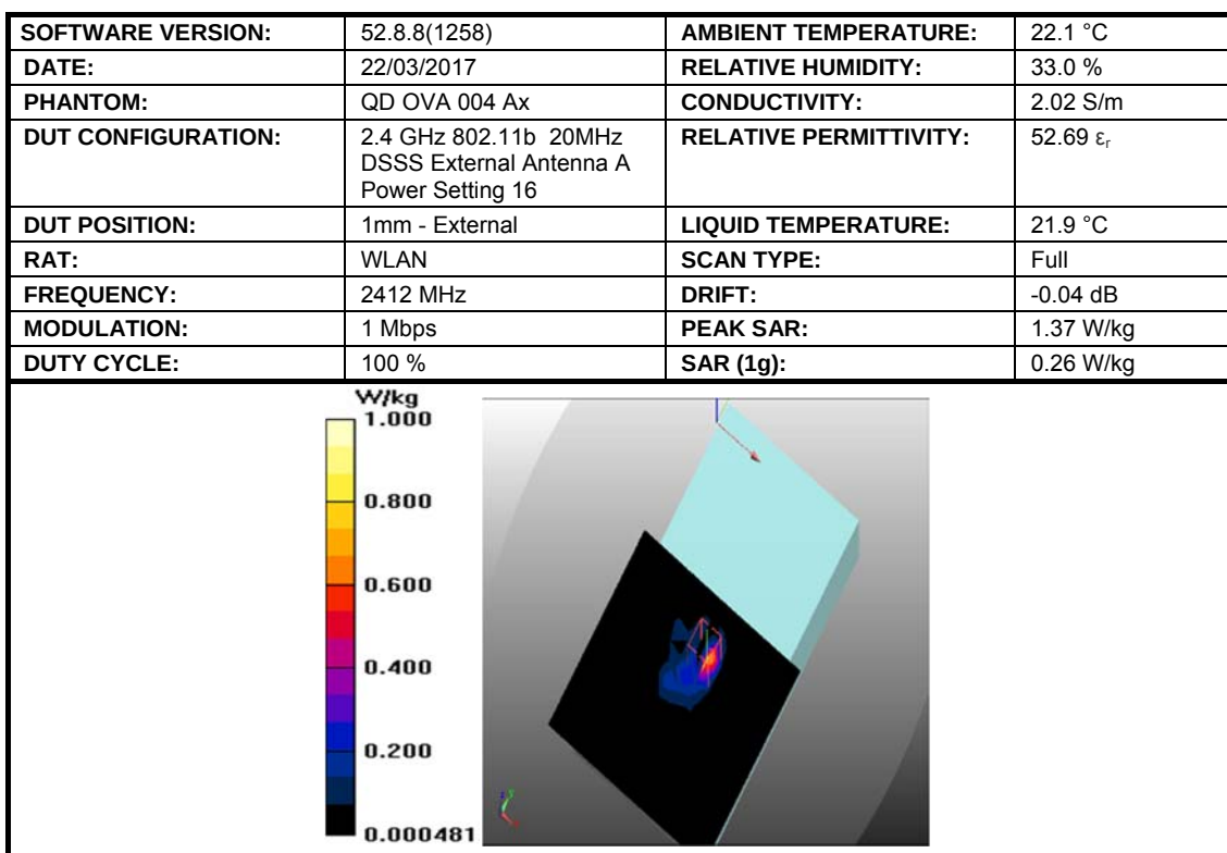
Figure 4: SAR Body-Extremity Testing Results for the DAQRI Smart Helmet at 2412 MHz.
