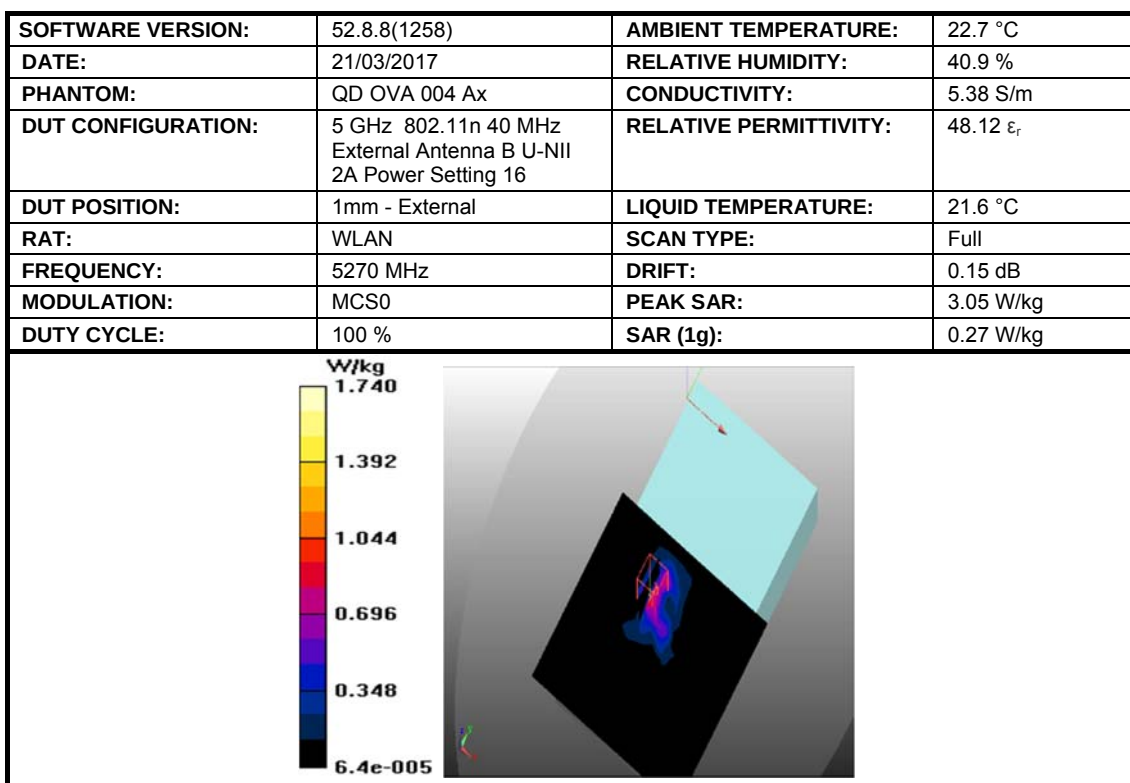
Figure 9: SAR Body-Extremity Testing Results for the DAQRI Smart Helmet at 5270 MHz.
