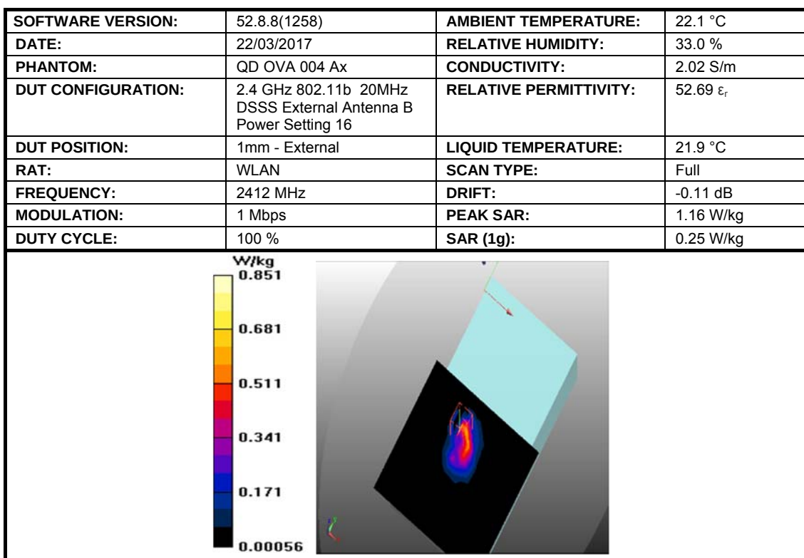
Figure 5: SAR Body-Extremity Testing Results for the DAQRI Smart Helmet at 2412 MHz.
