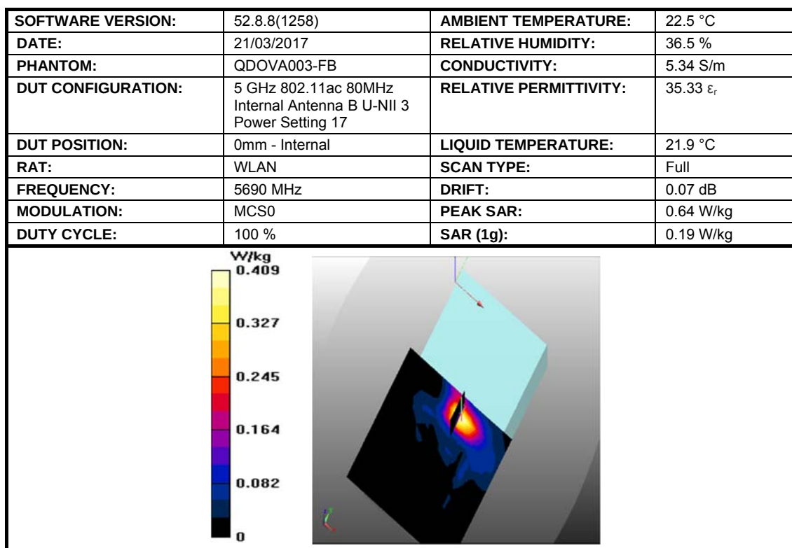
Figure 15: SAR Head Testing Results for the DAQRI Smart Helmet at 5690 MHz.
