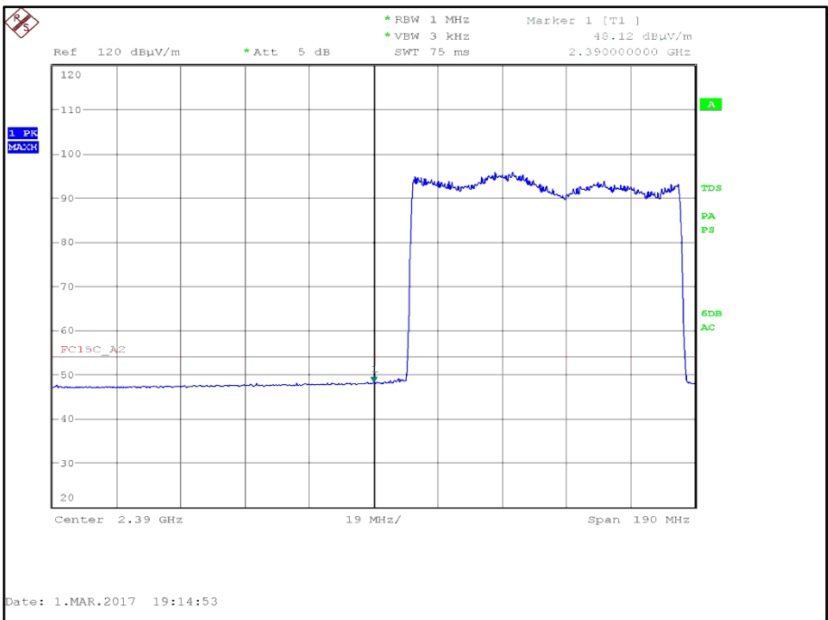
Figure 44 - 2402 MHz, Hopping, \pi/4 DQPSK, Measured Frequency 2390.0 MHz, Average
