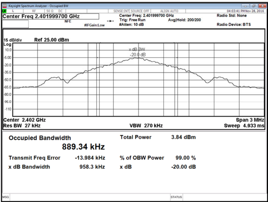
Figure 11 - 2402 MHz - GFSK
