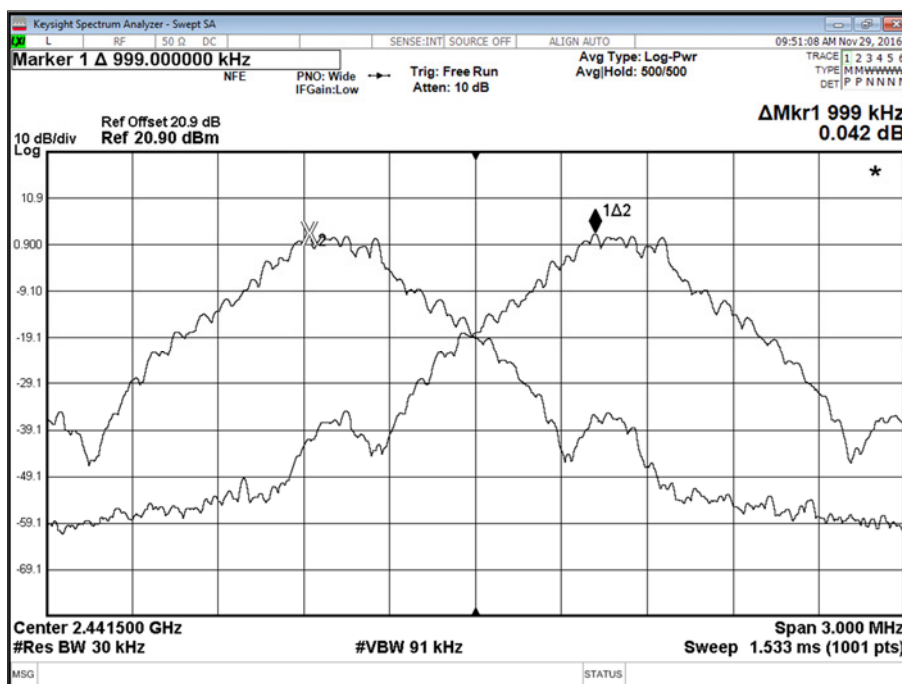
Figure 7 - GFSK
