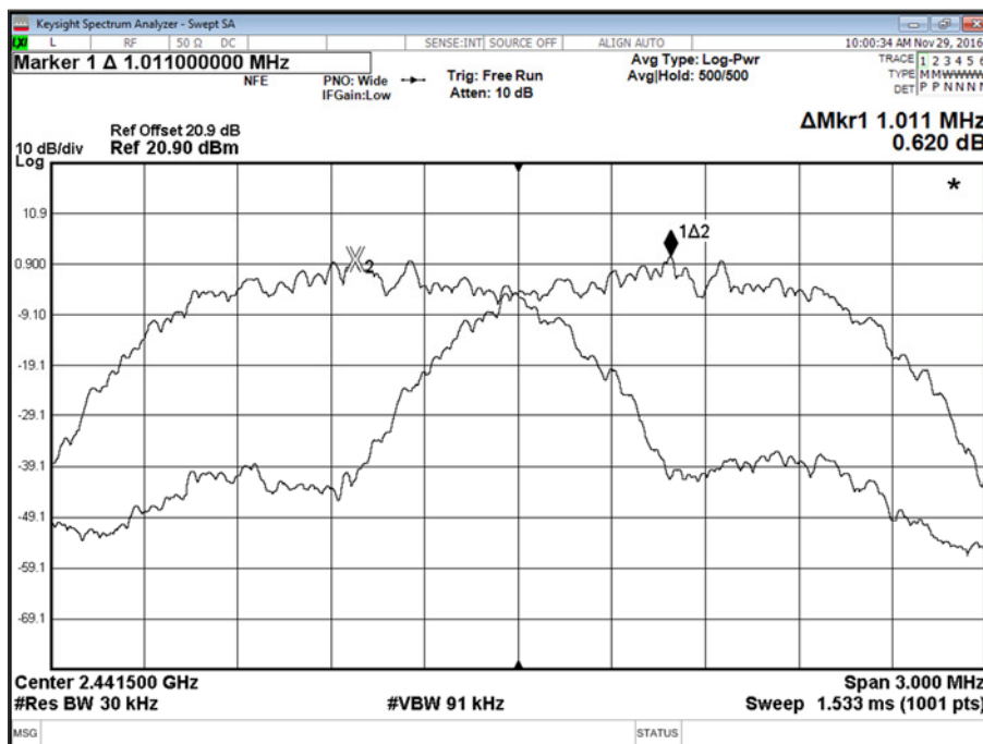
Figure 8 - \pi/4 DQPSK
