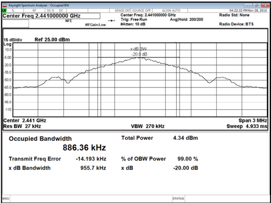
Figure 14 - 2441 MHz - GFSK
