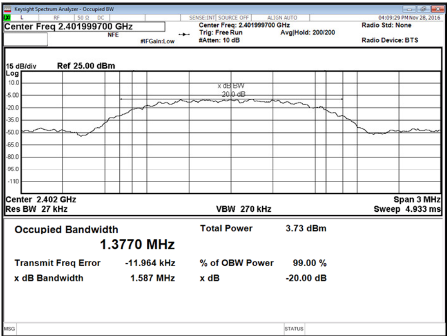
Figure 13 - 2402 MHz - 8-DPSK
