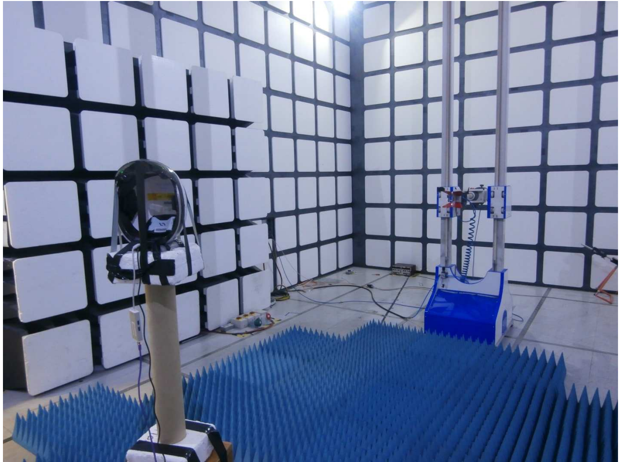
FCC Part Radiated Emissions 1 GHz to 18 GHz
