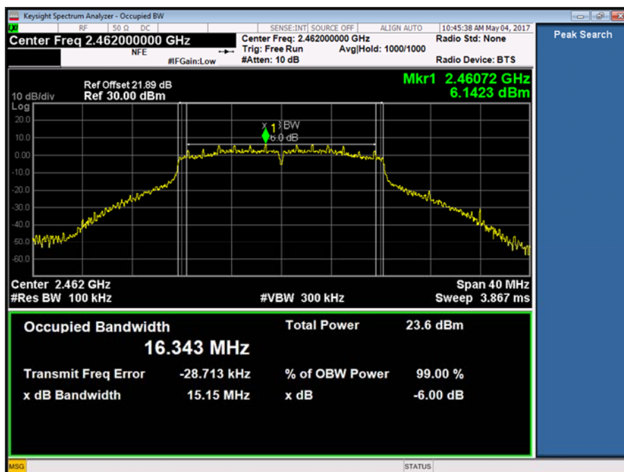
Figure 6 - 2462 MHz
