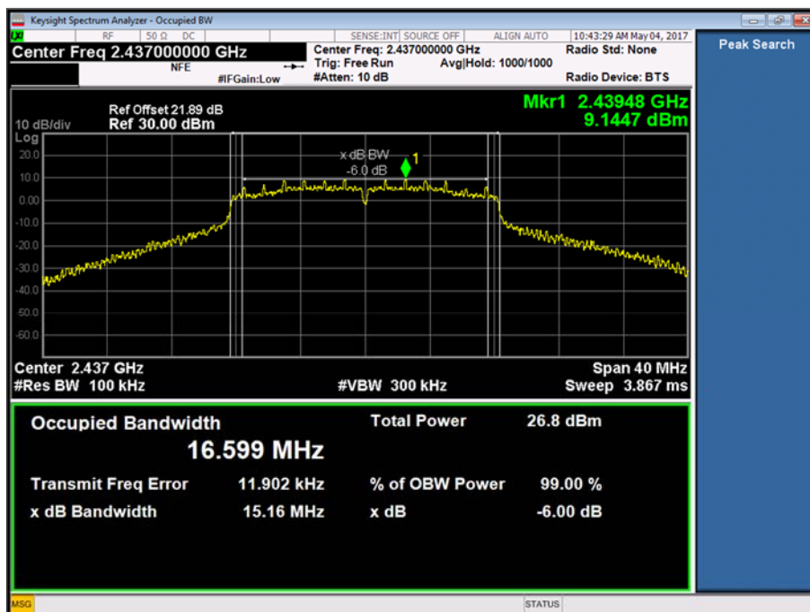
Figure 5 - 2437 MHz
