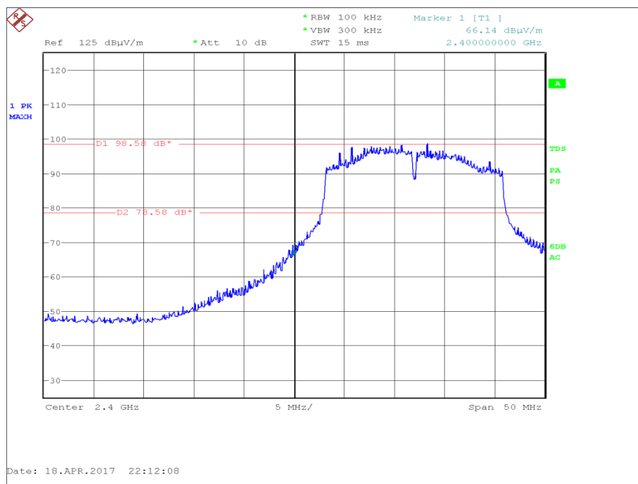
Figure 19 - Data Rate/MCS with Highest Power and Widest Bandwidth - MCS1 - 2412 MHz - Measured Frequency 2400.0 MHz
