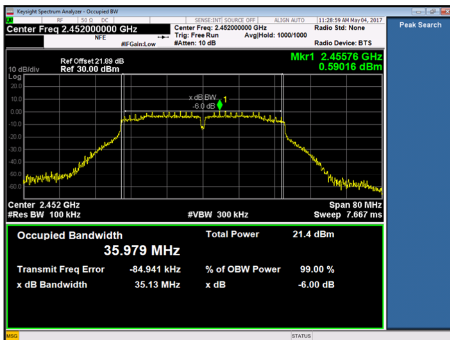
Figure 12 - 2452 MHz
