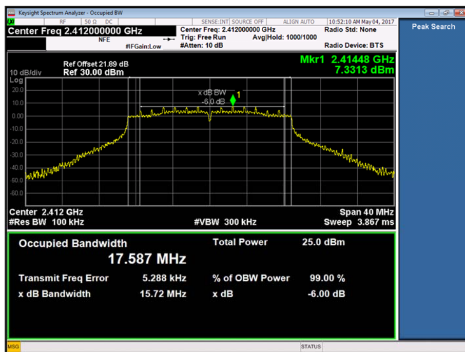
Figure 7 - 2412 MHz
