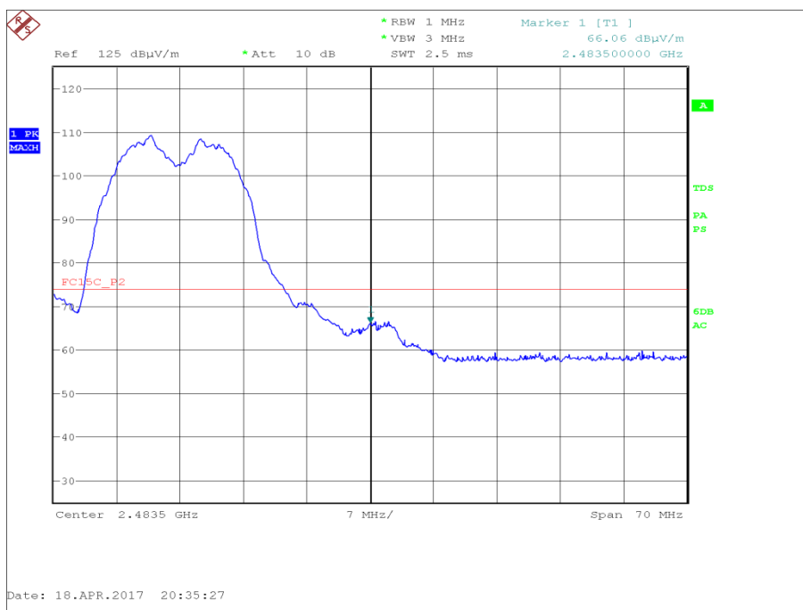
Figure 27 - Data Rate/MCS with Highest Power - 5.5 Mbps - 2462 MHz - Measured Frequency 2483.5 MHz - Peak
