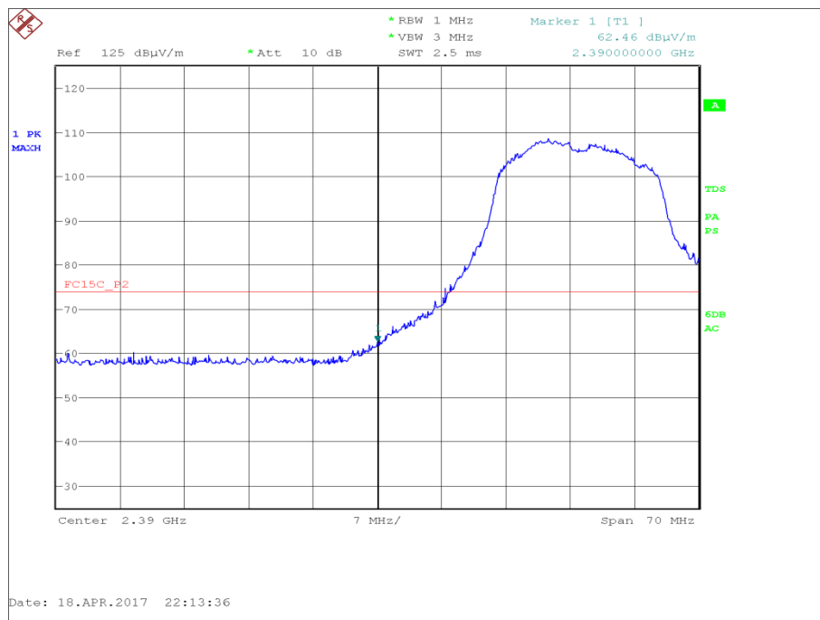
Figure 37 - Data Rate/MCS with Highest Power and Widest Bandwidth - MCS1 - 2412 MHz - Measured Frequency 2390.0 MHz - Peak
