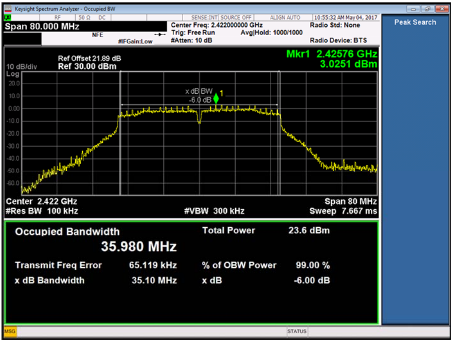
Figure 10 - 2422 MHz
