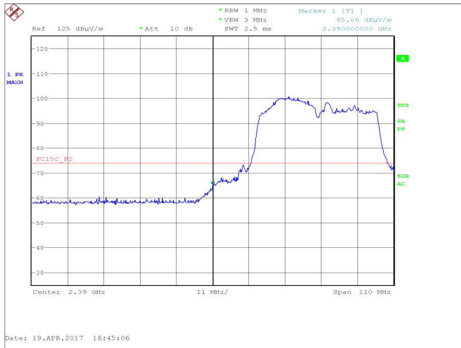
Figure 41 - Data Rate/MCS with Highest Power - MCS2 - 2422 MHz - Measured Frequency 2390.0 MHz - Peak
