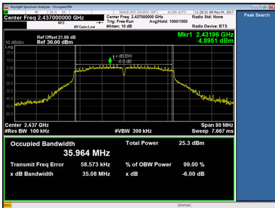
Figure 11 - 2437 MHz
