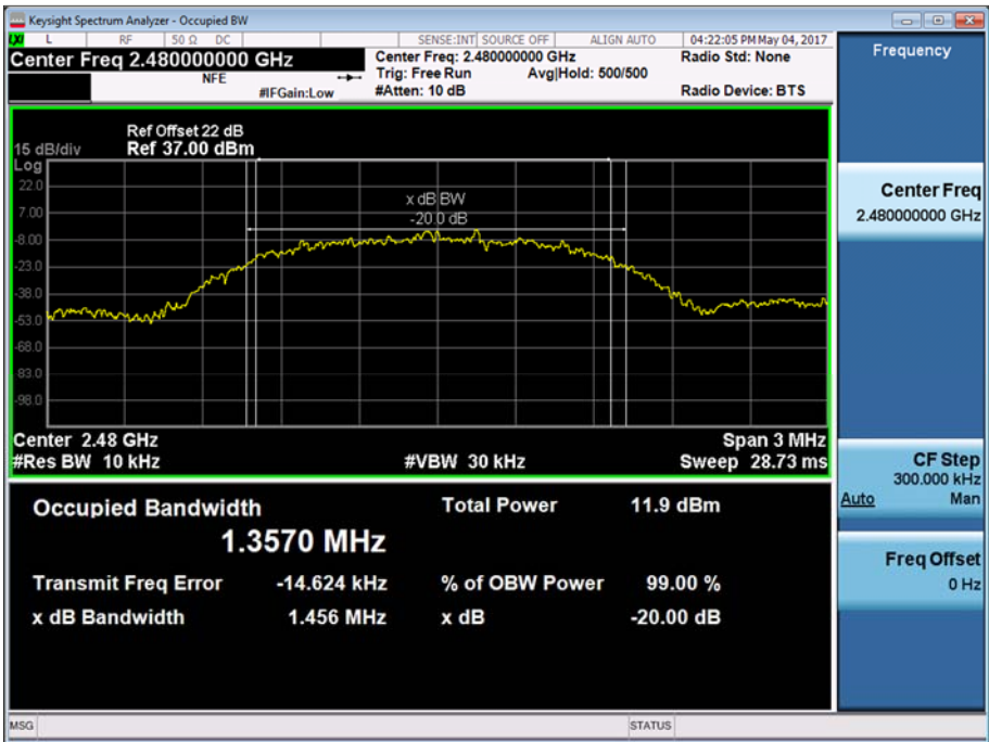
Figure 10 - 2480 MHz - 8-DPSK
