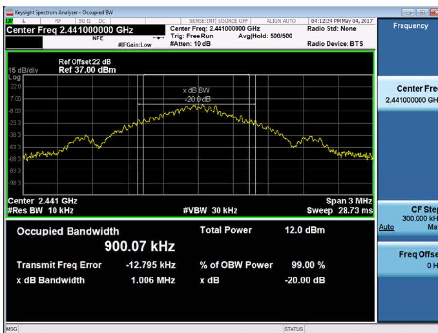
Figure 5 - 2441 MHz - GFSK
