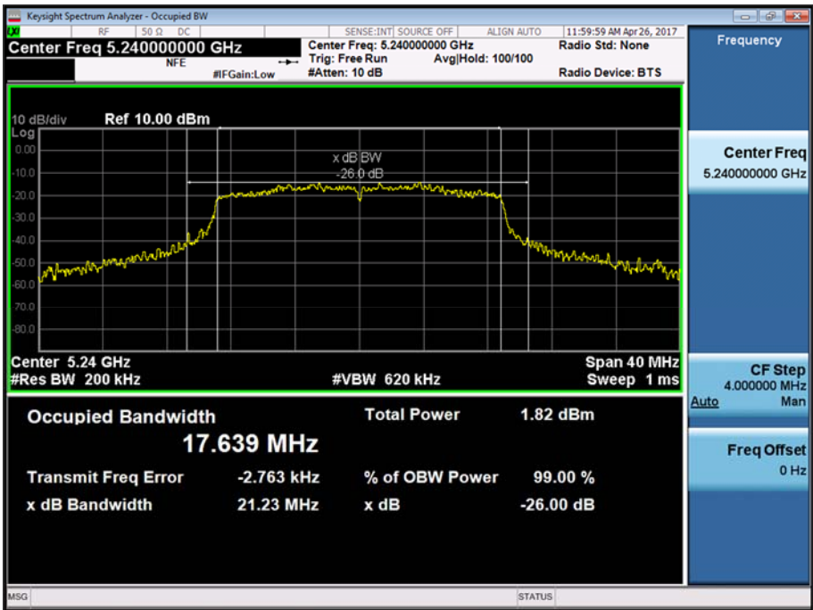
Figure 17 - U-NII 1 - 5240 MHz - 26 dB Bandwidth
