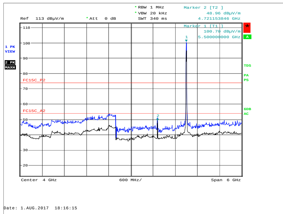
Figure 1 - U-NII 2c - 5500 MHz - 1 GHz to 7 GHz - Horizontal and Vertical
