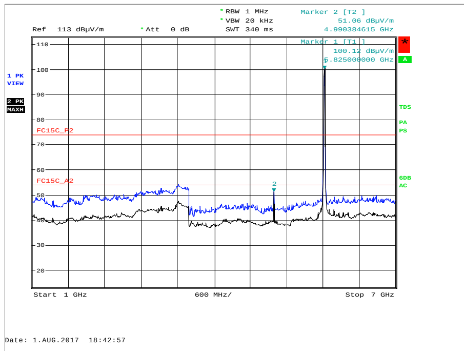
Figure 6 - U-NII 3 - 5825 MHz - 1 GHz to 7 GHz - Horizontal and Vertical
