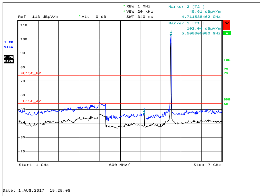
Figure 13 - U-NII 2c - 5500 MHz - 1 GHz to 7 GHz - Horizontal and Vertical
