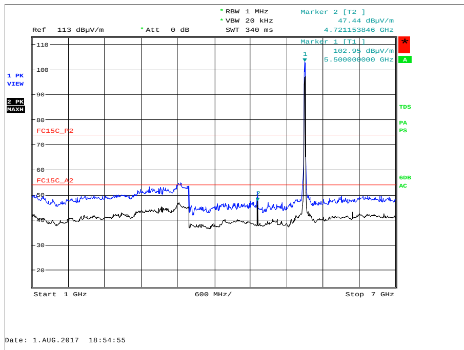
Figure 7 - U-NII 2c - 5500 MHz - 1 GHz to 7 GHz - Horizontal and Vertical
