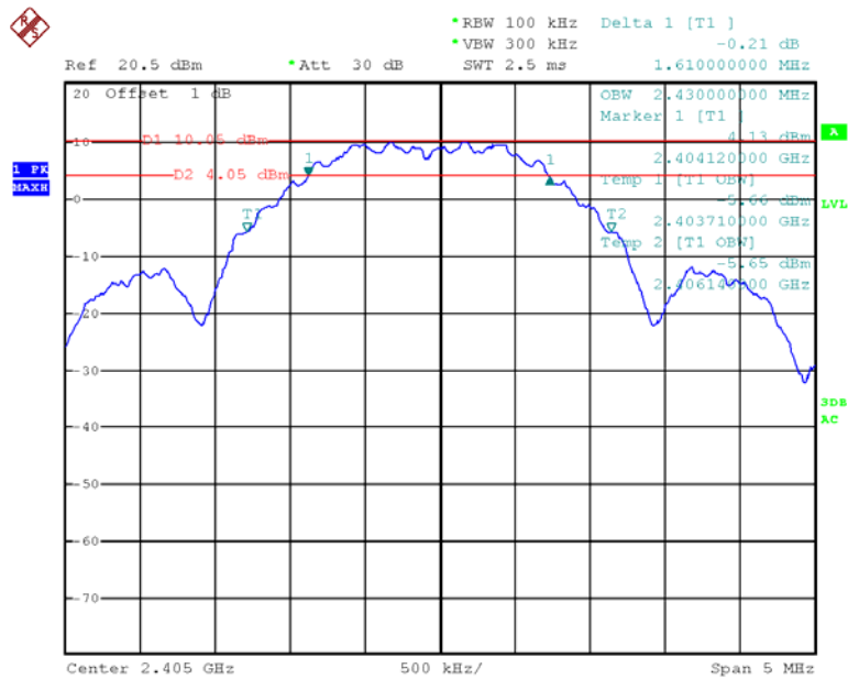
Low Channel-2405MHz
