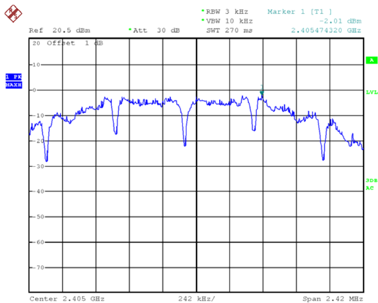
Power Spectral Density, Low Channel-2405MHz
