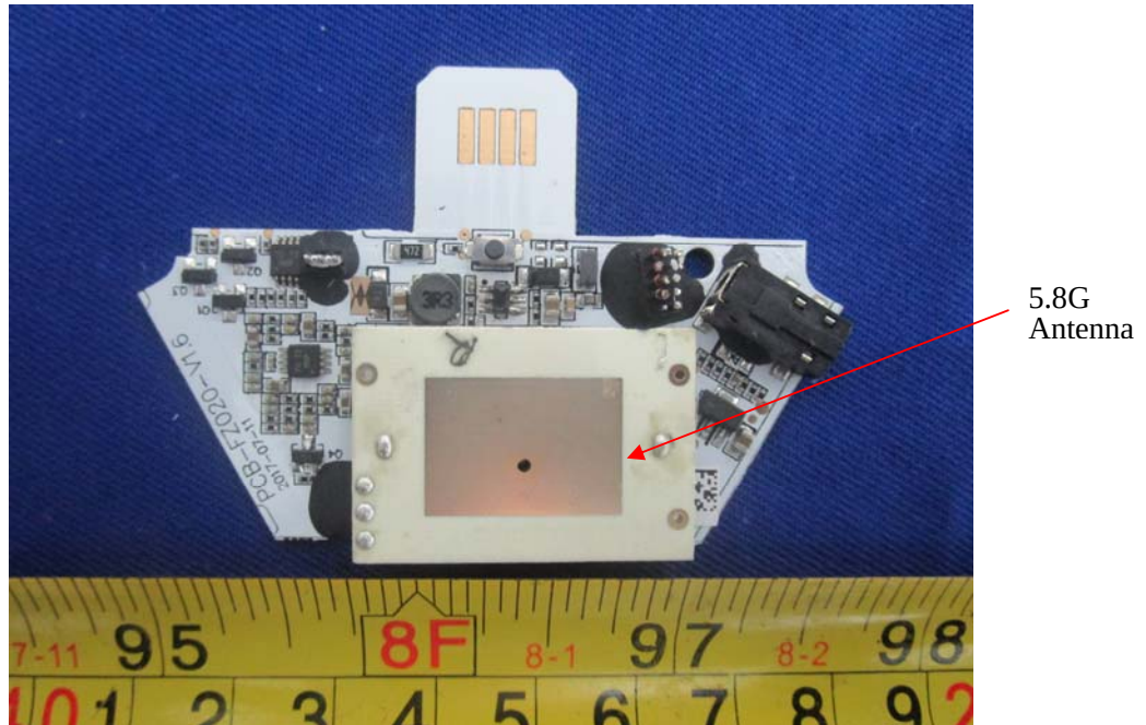
EUT –PCB-FZ020 Top View
