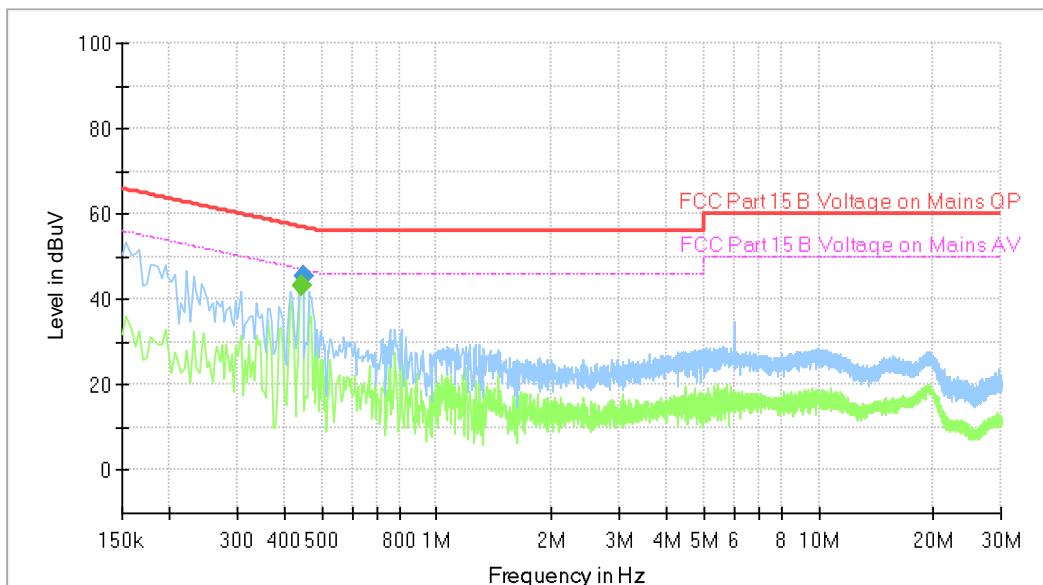
Full Spectrum
