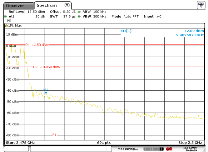
Hopping mode
