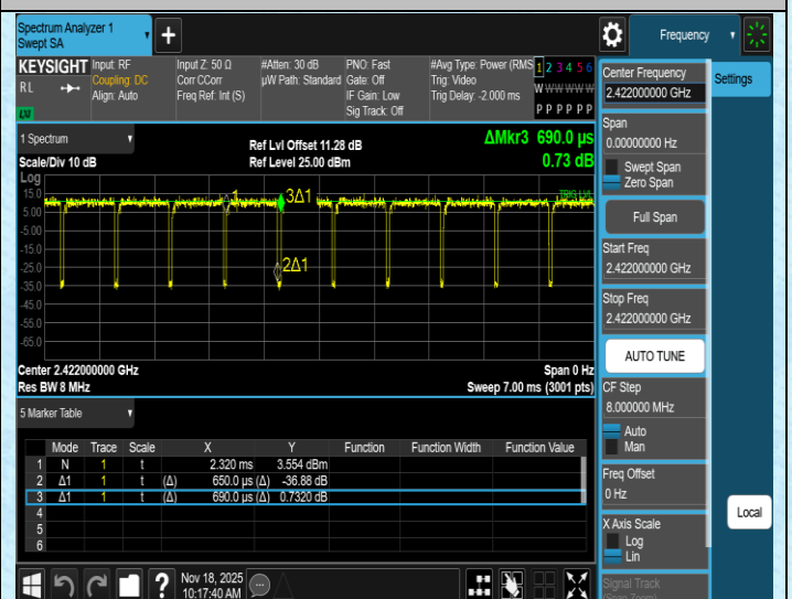
NTNV-11N40SISO-Ant1-2422
