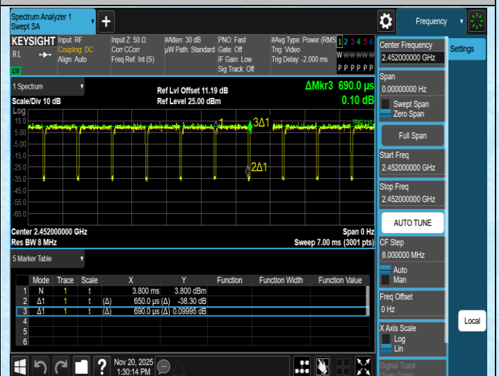
NTNV-11N40SISO-Ant1-2452
