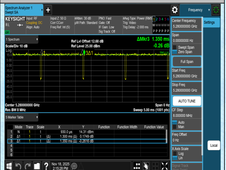
NTNV-11N20SISO-Ant1-5280
