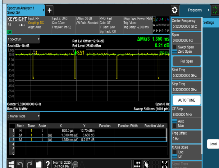
NTNV-11N20SISO-Ant1-5320
