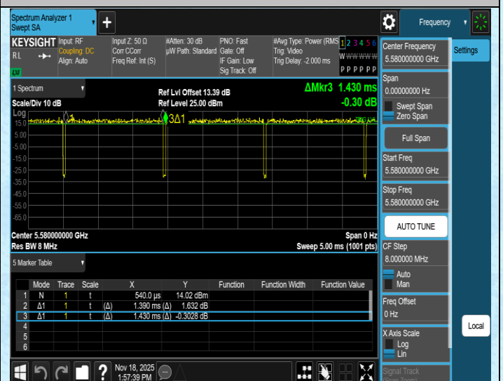
NTNV-11A-Ant1-5580
