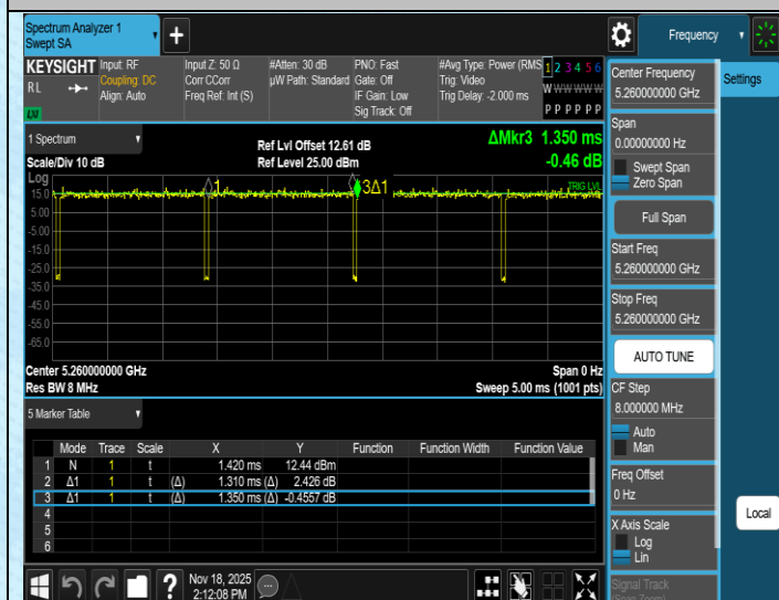
NTNV-11N20SISO-Ant1-5260
