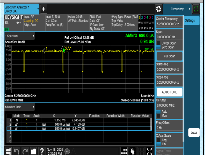
NTNV-11N40SISO-Ant1-5230
