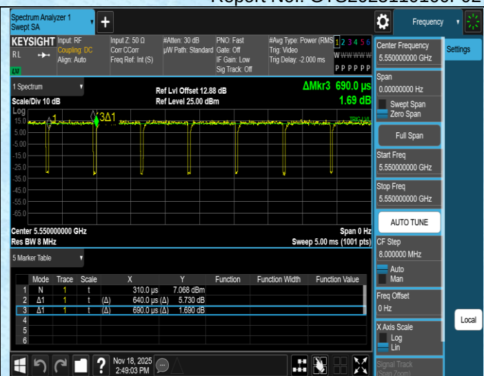
NTNV-11N40SISO-Ant1-5550
