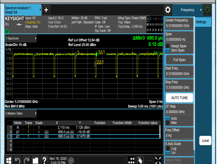
NTNV-11N40SISO-Ant1-5310
