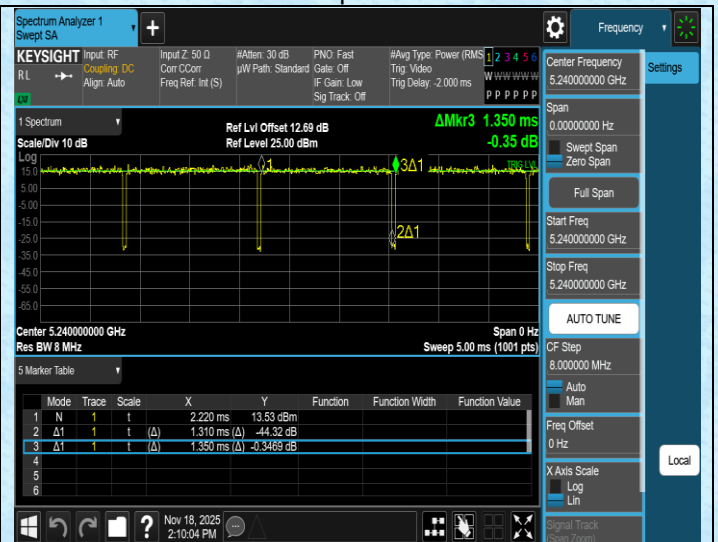
NTNV-11N20SISO-Ant1-5240
