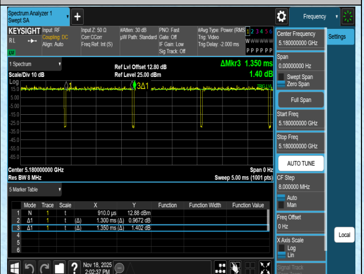
NTNV-11N20SISO-Ant1-5180
