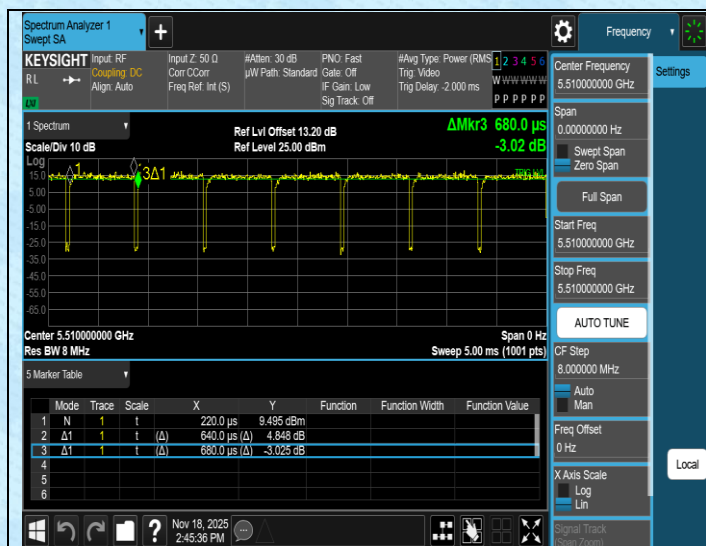
NTNV-11N40SISO-Ant1-5510
