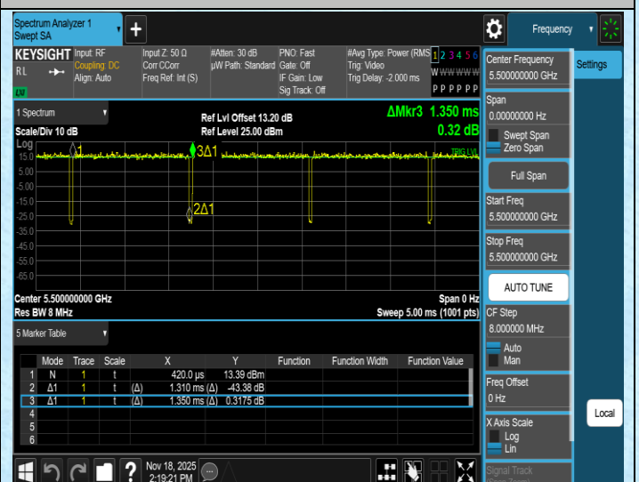
NTNV-11N20SISO-Ant1-5500
