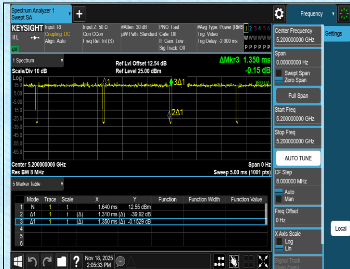
NTNV-11N20SISO-Ant1-5200
