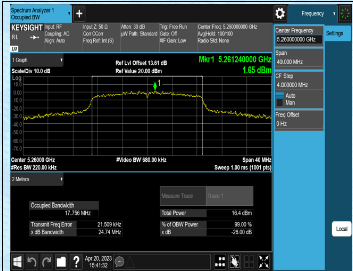
11AC20SISO-Ant1-5260
