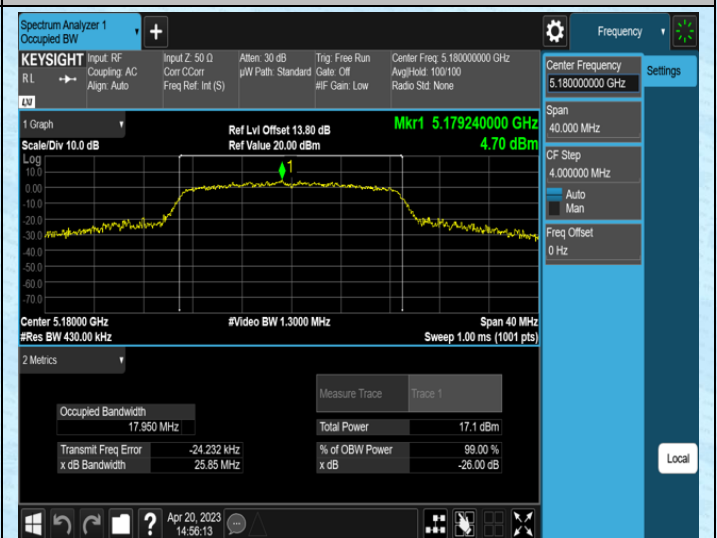
11N20SISO-Ant1-5180
