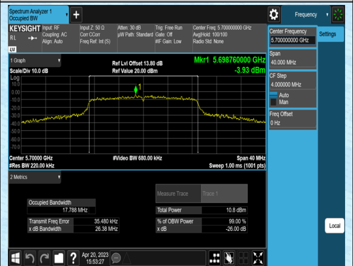
11AC20SISO-Ant1-5700
