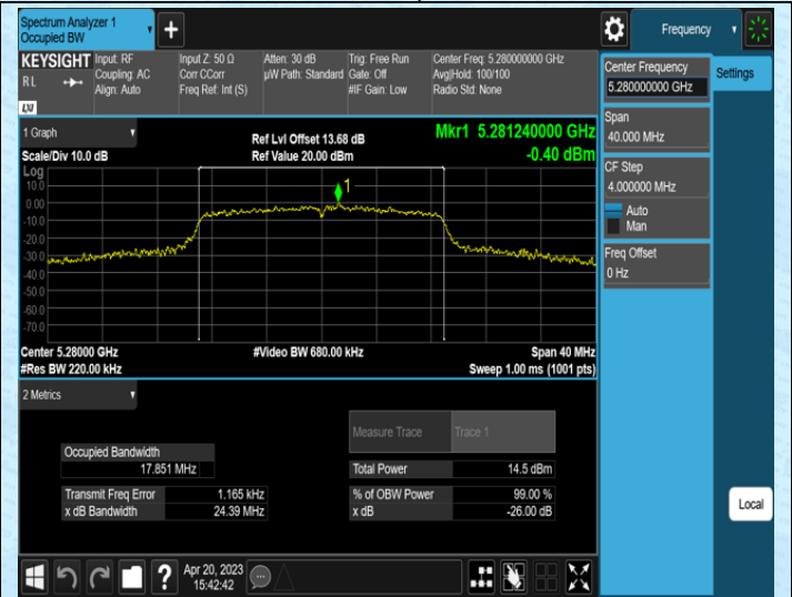
11AC20SISO-Ant1-5280
