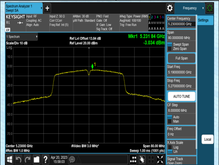
11AC40SISO-Ant1-5230
