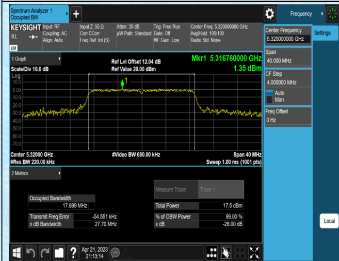
11AC20SISO-Ant1-5320
