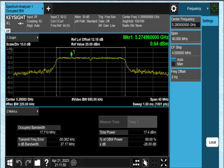
11AC20SISO-Ant1-5280
