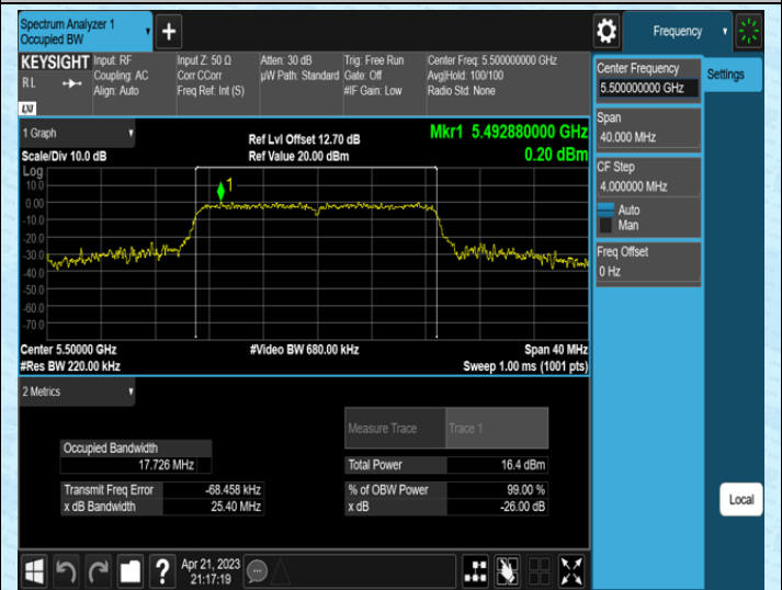
11AC20SISO-Ant1-5500
