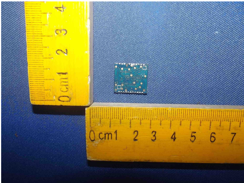
Figure 19 PCB of the EUT-Back View
