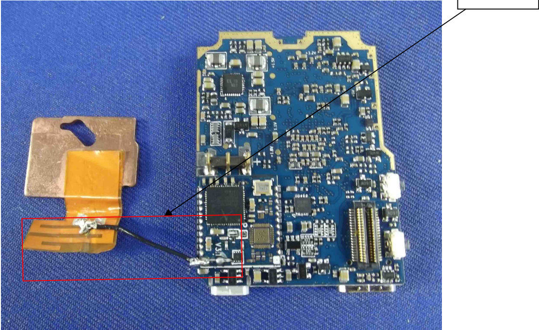
Figure 13 PCB of the EUT-Antenna View
