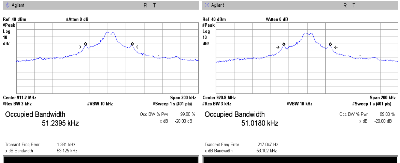
Plot 7.2.1 Occupied bandwidth test result
