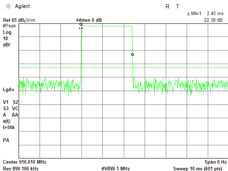
Plot 7.1.21 Transmission pulse duration
