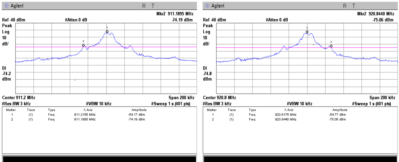
Plot 7.2.2 Cross point frequencies, low and high band edges
