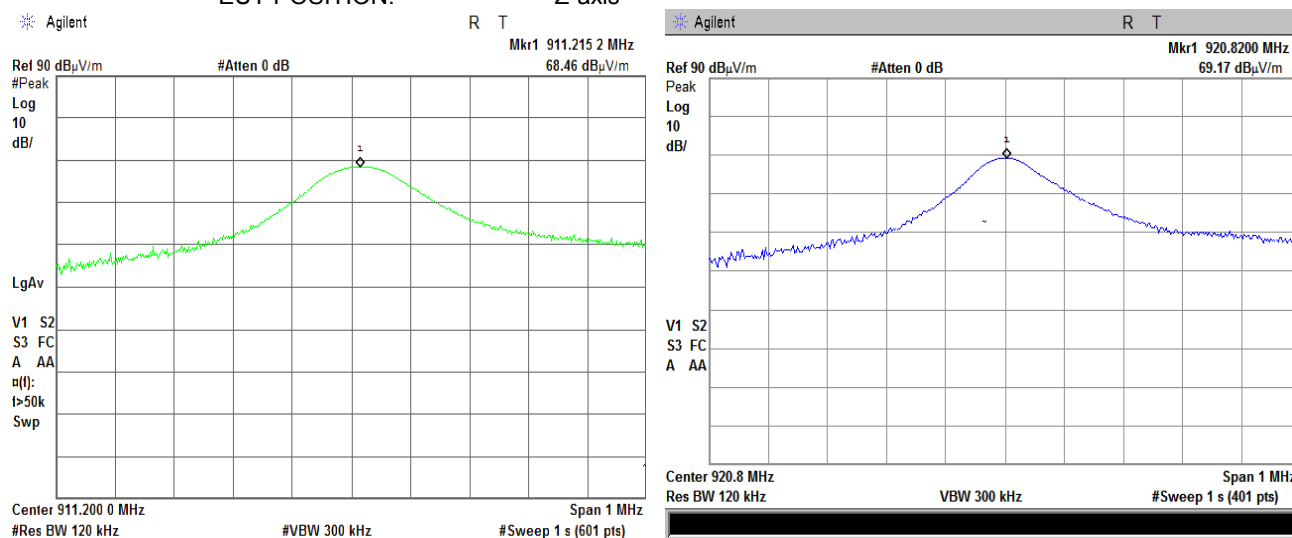
Plot 7.1.4 Radiated emission measurements at the fundamental frequency
