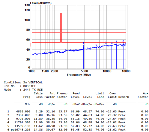
2.4G_SRD_MID_TX_Vertical
