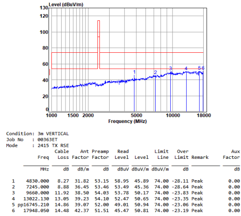
2.4G_SRD_LOW_TX_Vertical
