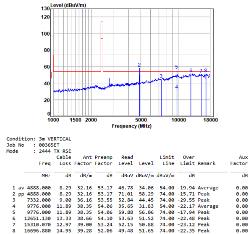
2.4G_SRD_MID_TX_Vertical
