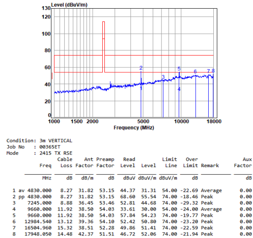
2.4G_SRD_LOW_TX_Vertical
