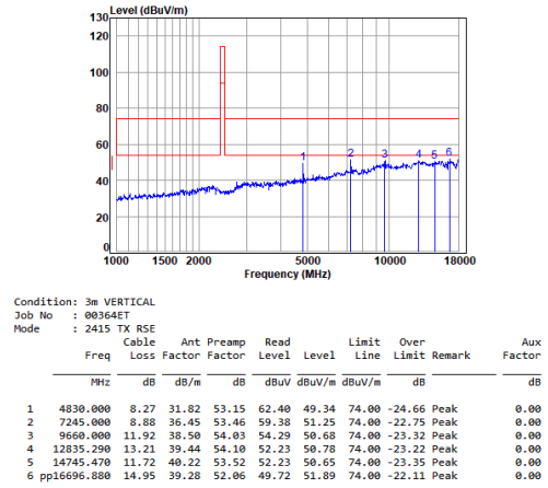
2.4G_SRD_LOW_TX_Vertical
