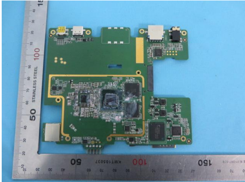
(7) EUT Photo
