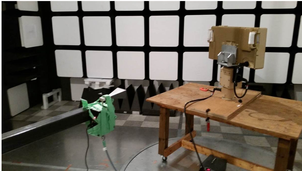
Radiated Emissions 18 GHz to 26 GHz scan
