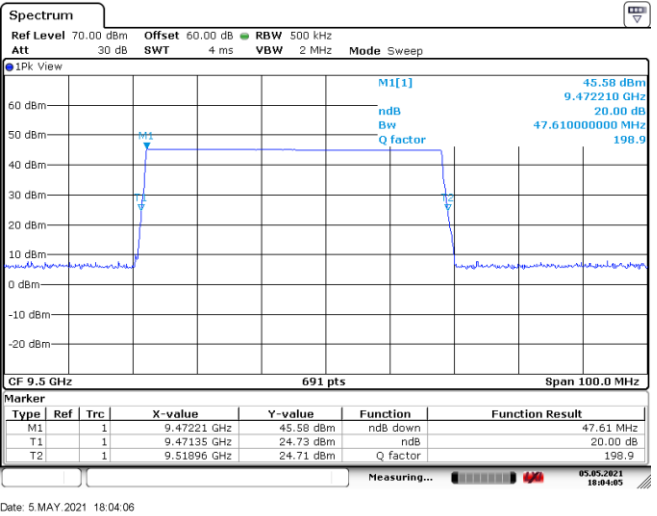
Figure 8.3-11: 20dB bandwidth, tx on mid channel with sweeping turned on
