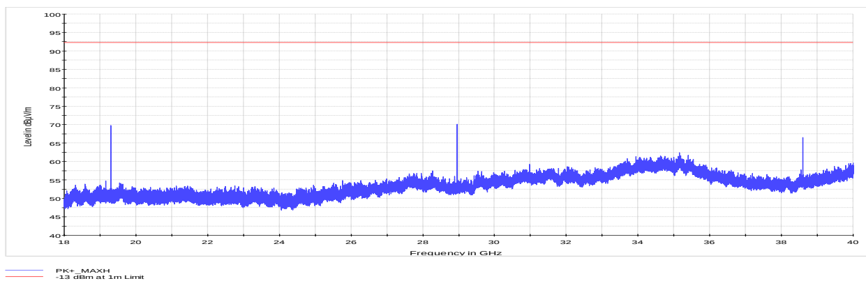
Figure 8.5-9: Cabinet radiated Spurious emissions 18 to 40 GHz, Tx @ high channel
