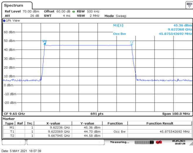
Figure 8.3-9: 99% bandwidth, tx on high channel with sweeping turned on
