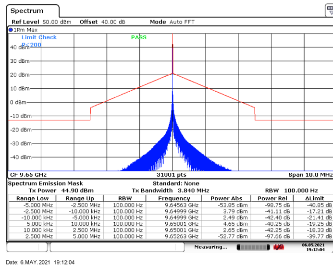
Figure 8.4-3: Emission mask at high channel
