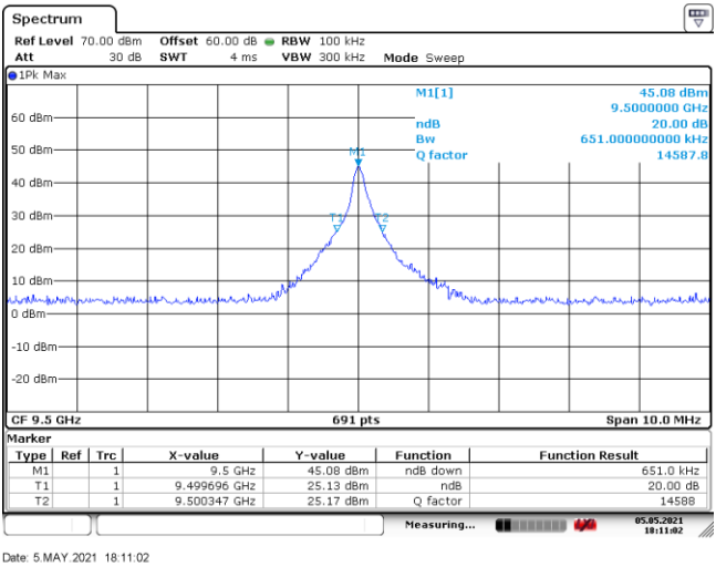
Figure 8.3-5: 20dB bandwidth, tx on mid channel with sweeping turned off
