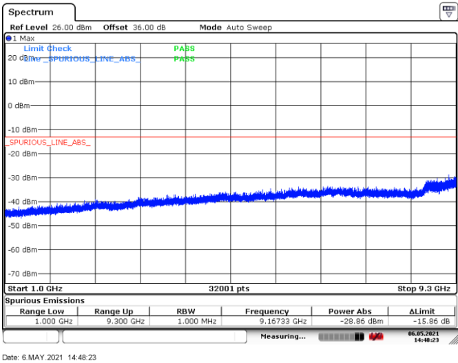
Figure 8.4-7: Conducted spurious emissions 1 to 9.3 GHz, Tx on low channel
