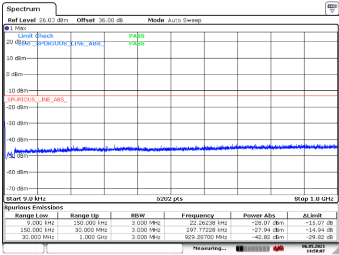
Figure 8.4-6: Conducted spurious emissions below 1 GHz, Tx on high channel
