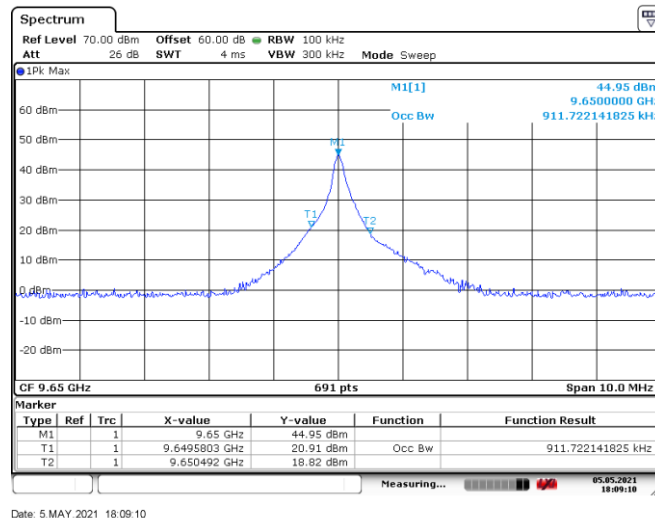
Figure 8.3-3: 99% bandwidth, tx on high channel with sweeping turned off
