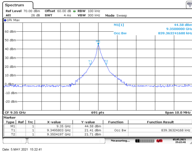
Figure 8.3-1: 99% bandwidth, tx on low channel with sweeping turned off
