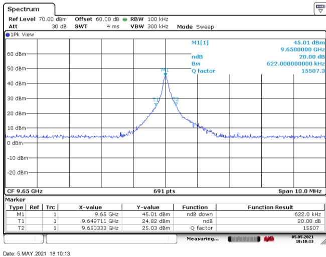
Figure 8.3-6: 20dB bandwidth, tx on high channel with sweeping turned off
