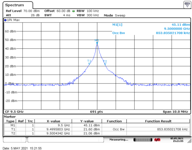
Figure 8.3-2: 99% bandwidth, tx on mid channel with sweeping turned off
