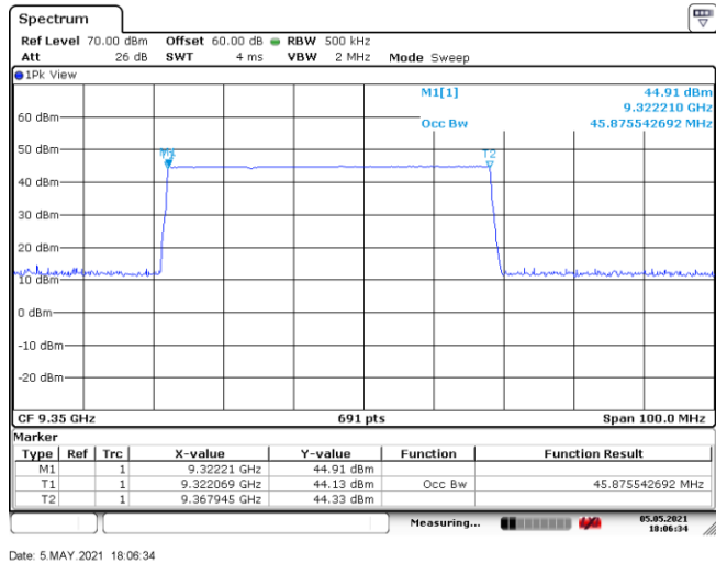
Figure 8.3-7: 99% bandwidth, tx on low channel with sweeping turned on
