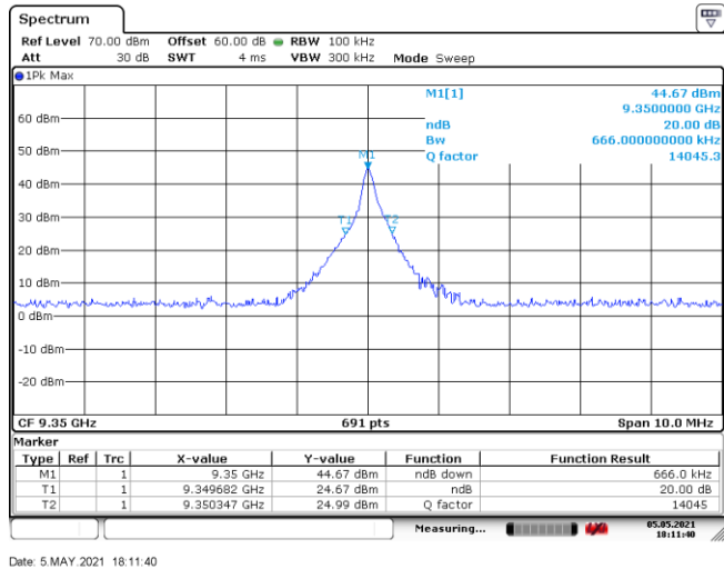
Figure 8.3-4: 20dB bandwidth, tx on low channel with sweeping turned off
