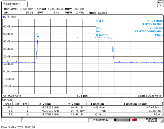
Figure 8.3-10: 20dB bandwidth, tx on low channel with sweeping turned on
