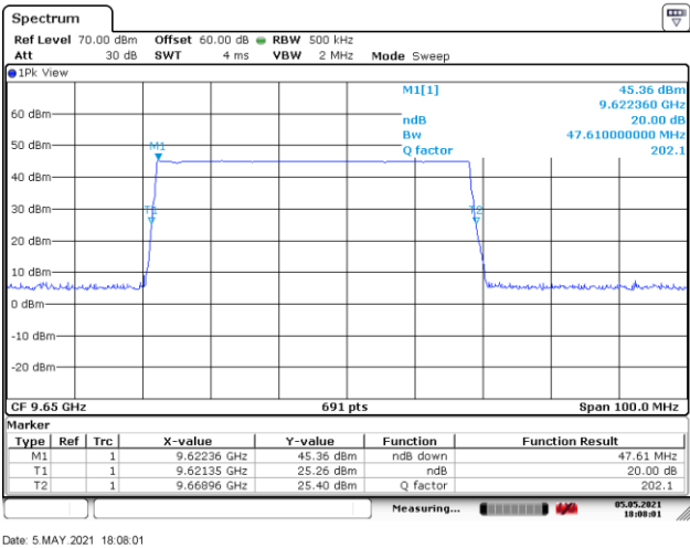
Figure 8.3-12: 20dB bandwidth, tx on high channel with sweeping turned on
