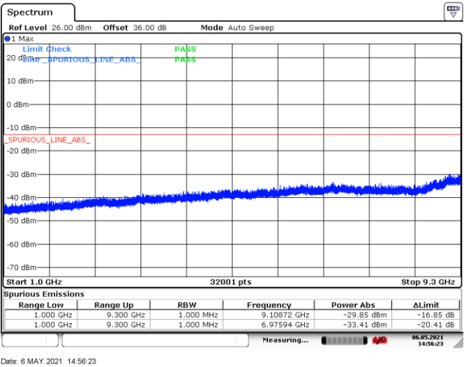
Figure 8.4-8: Conducted spurious emissions 1 to 9.3 GHz, Tx on mid channel
