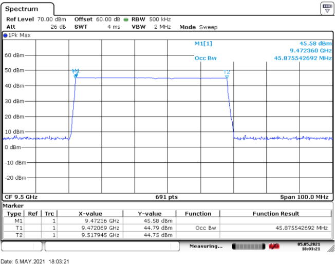
Figure 8.3-8: 99% bandwidth, tx on mid channel with sweeping turned on
