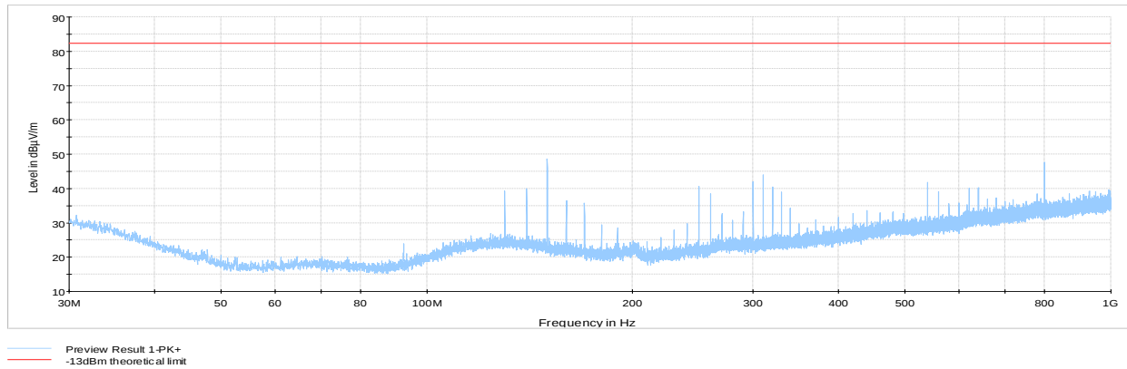
Figure 8.5-1: Cabinet radiated Spurious emissions within 30 to 1000 MHz, Tx @ low channel
