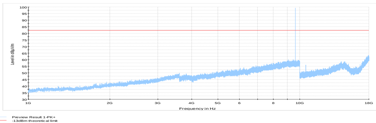
Figure 8.5-6: Cabinet radiated Spurious emissions 1 to 18 GHz, Tx @ high channel
