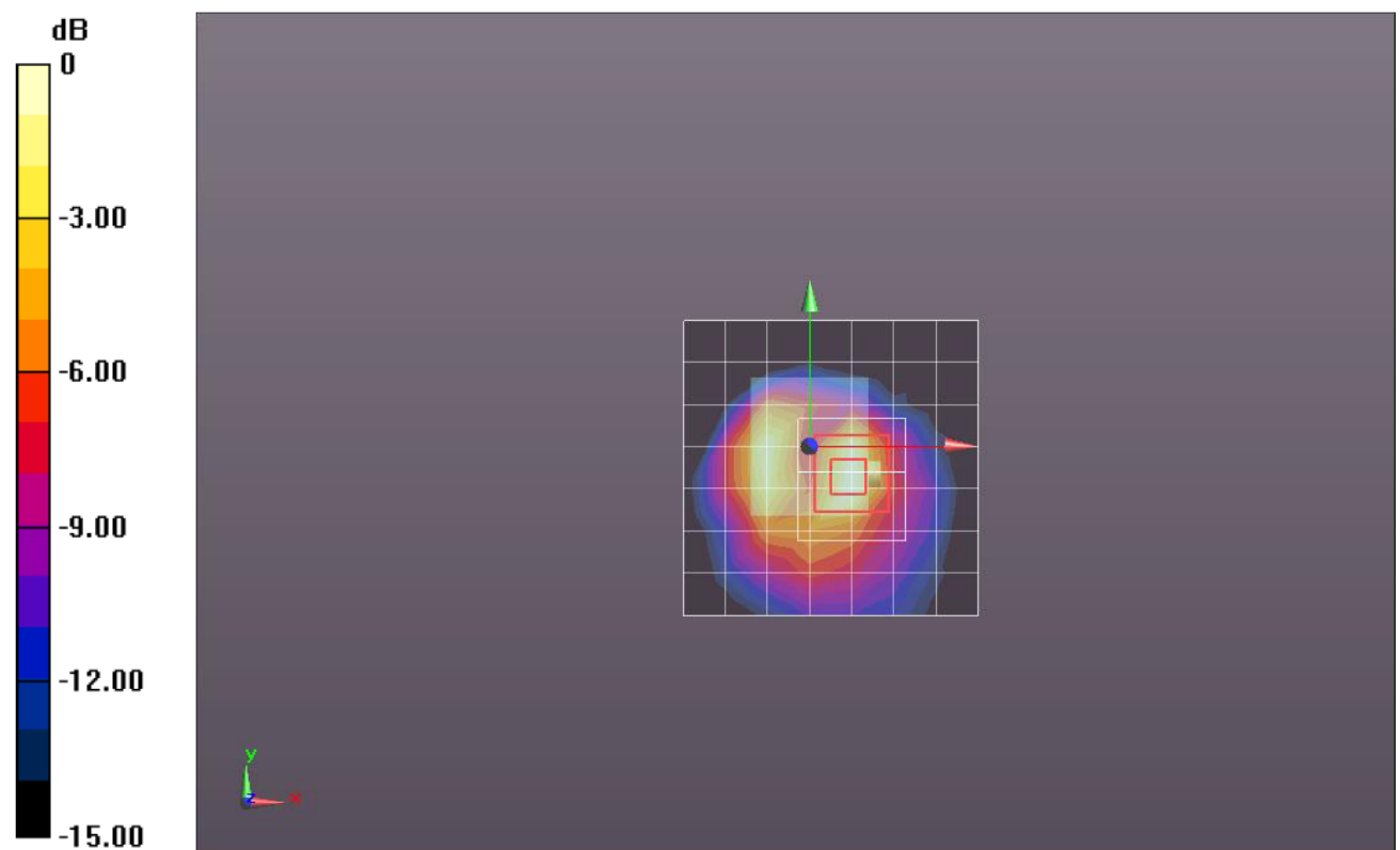
Plot 2: Body Wrist Worn (GSM850 Middle Channel)
