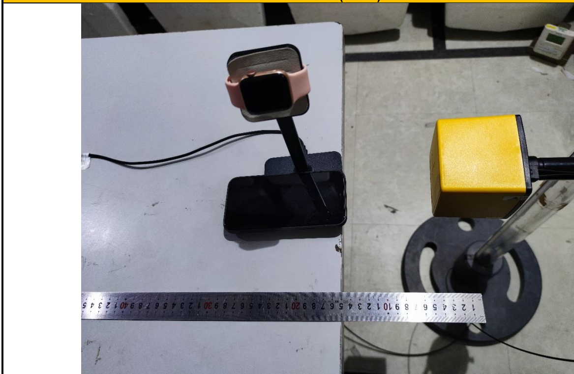
E-Field Strength and H-Field Strength Position A (15cm)
