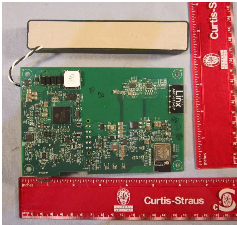
Internal Board Component Side
