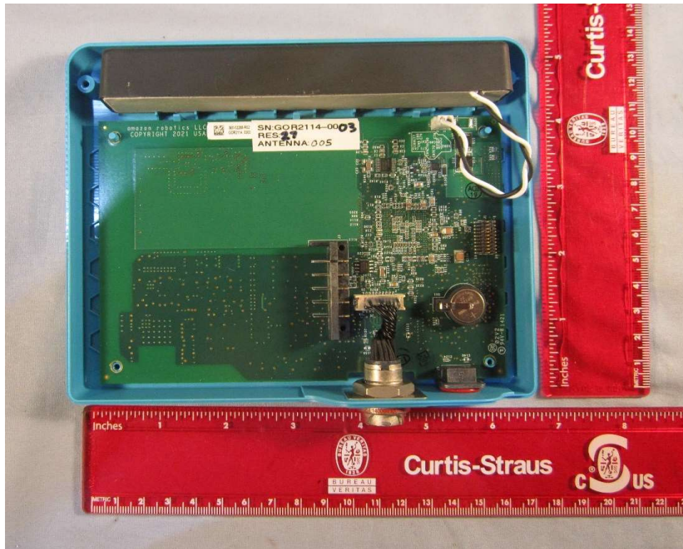
Back Cover of EUT Removed
