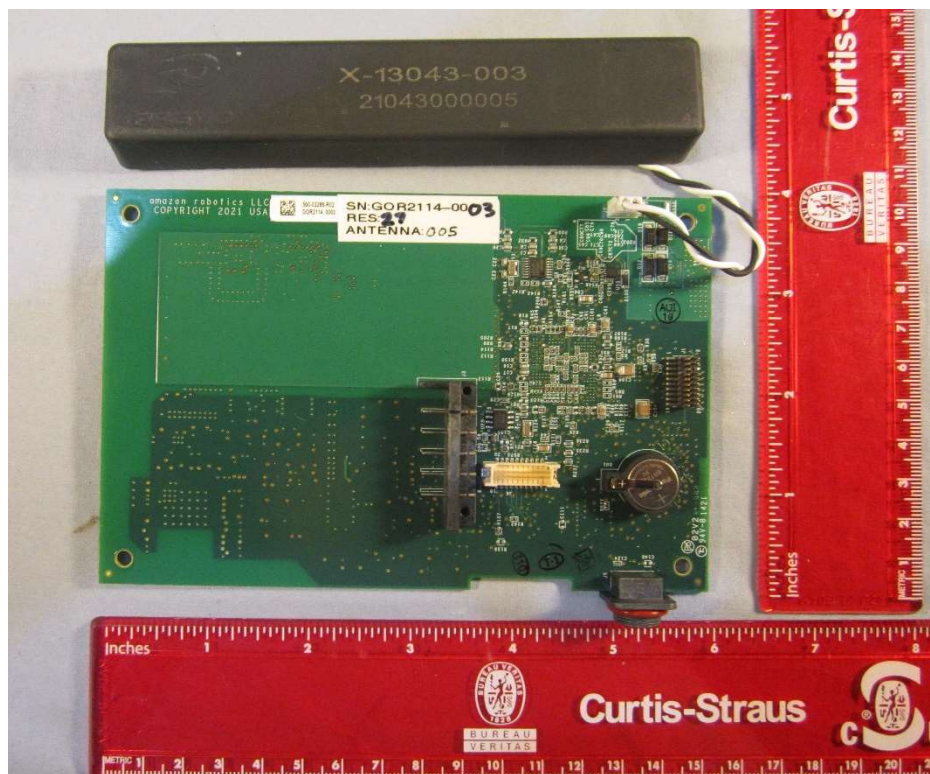
Internal Board Solder Side
