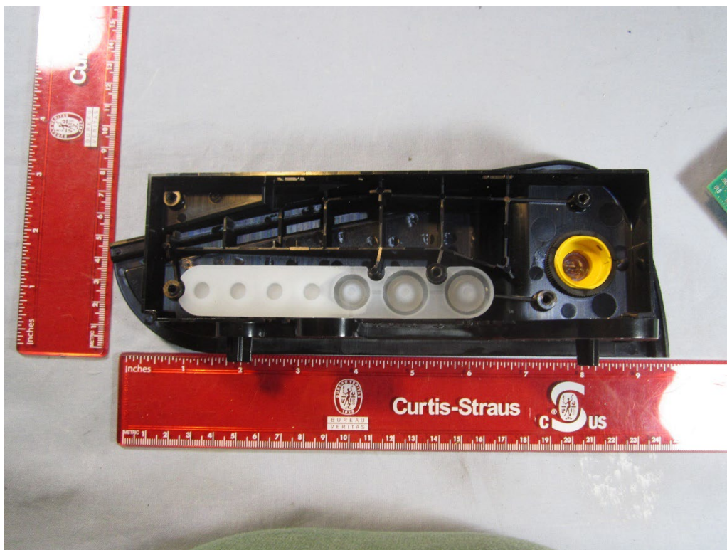
Back of Front Cover
