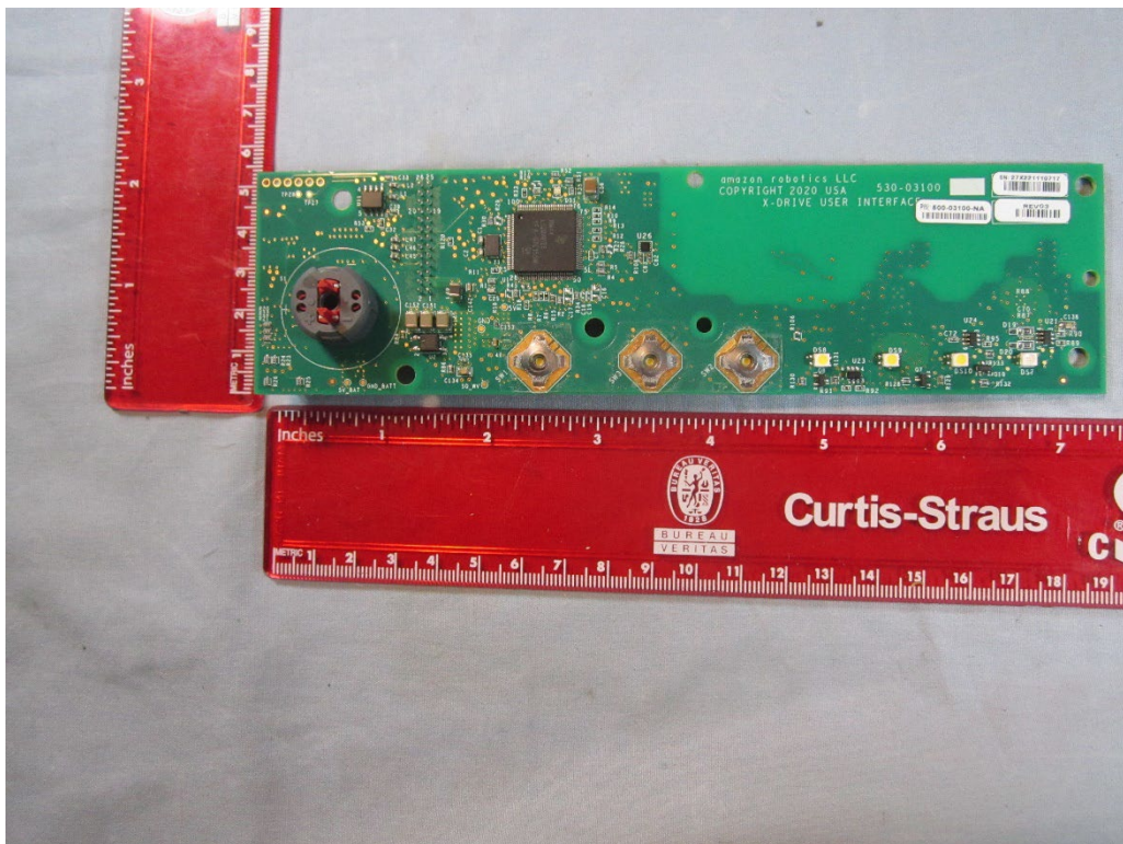
Rear of Internal Board
