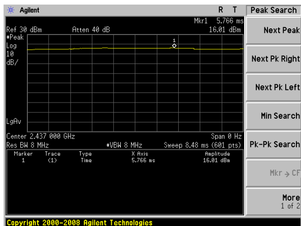
(802.11b) Duty Cycle plot on channel 6
