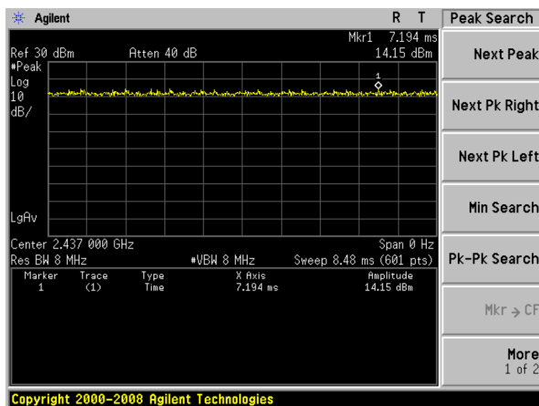
(802.11n40) Duty Cycle plot on channel 6
