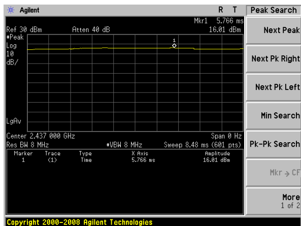
(802.11g) Duty Cycle plot on channel 6
