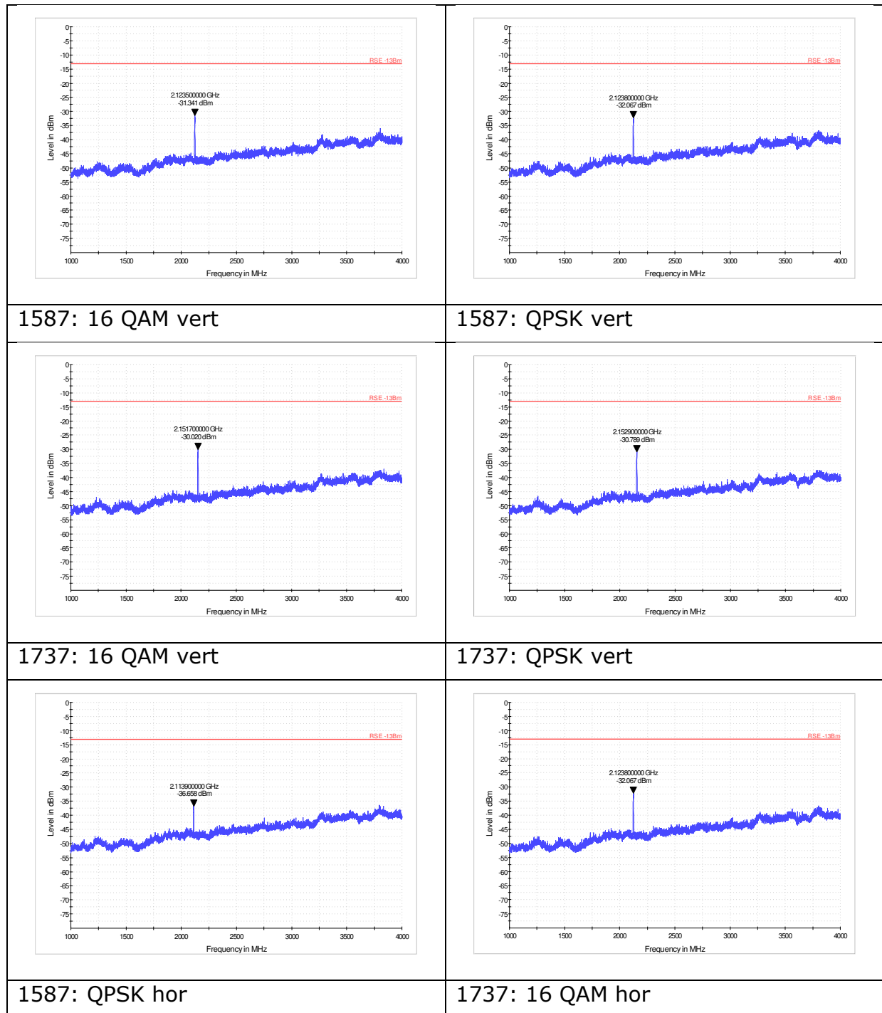
Figure 10: RSE pre-scans : 1 – 4 GHz
