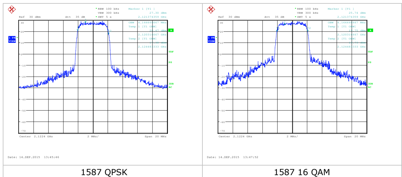
Figure 5: Occupied Bandwidth plots – worst case
