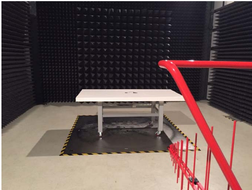
Spurious Emissions View (Below 1 GHz)
