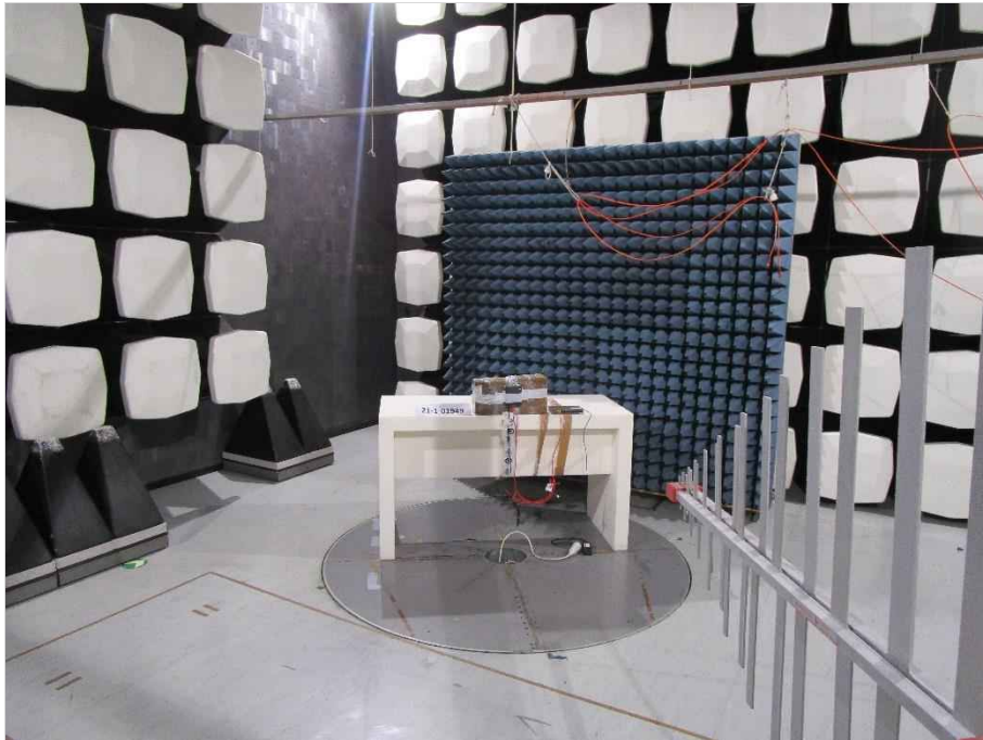
Photograph 2: EUT test setup in the semi anechoic chamber, close up view_EUT elevation 90°
