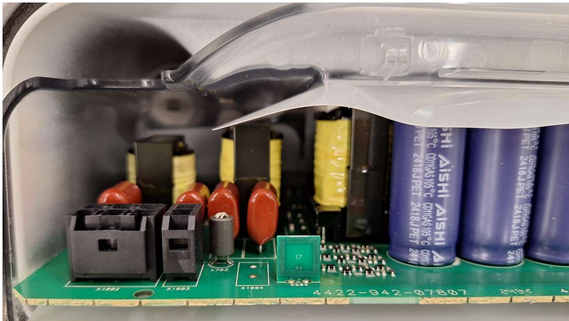
Photo 2 - internal view 2 (detail)
