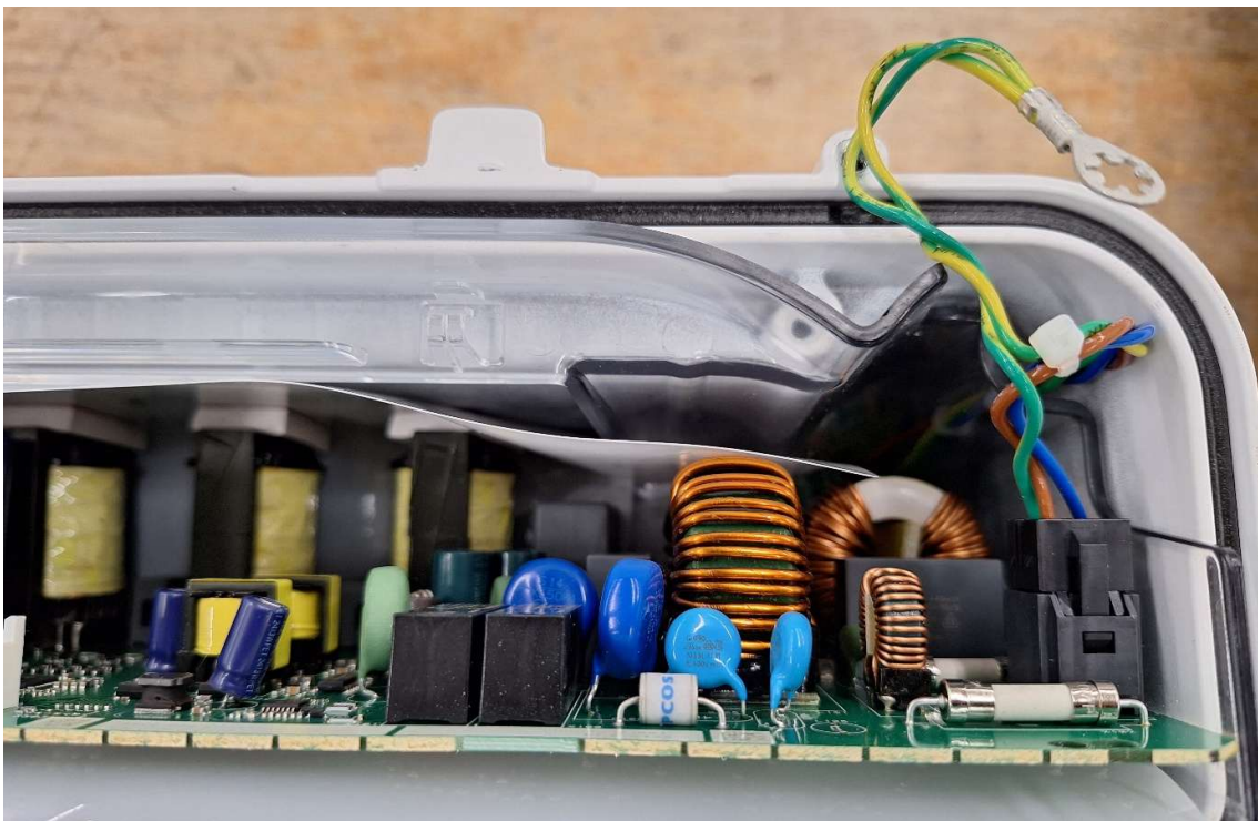
Photo 4 - internal view 4 (detail)
