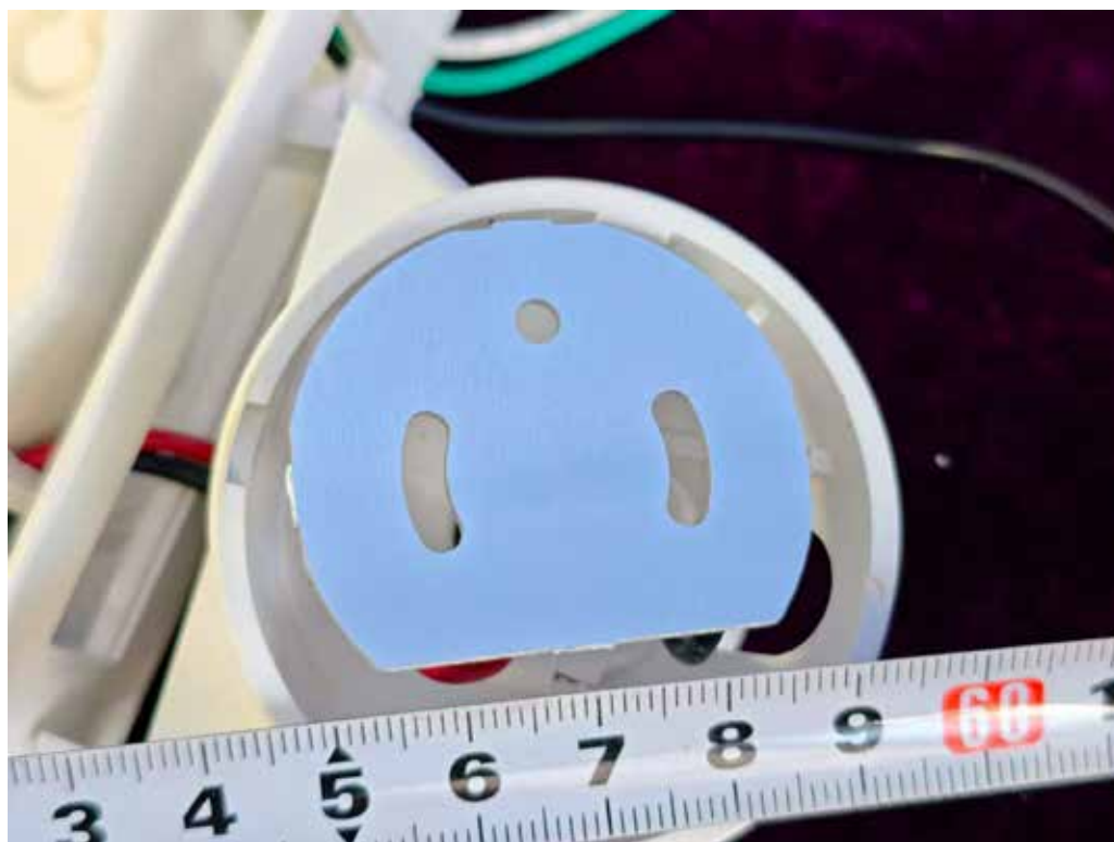
FIGURE 16 COMBO EXIT SIGN WITH FIRSTLINK (BCB4WFL1) BOARD4-2
