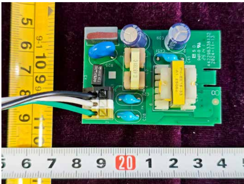
FIGURE 25 EXIT SIGN WITH FIRSTLINK (BXBWFL1) BOARD1-1
