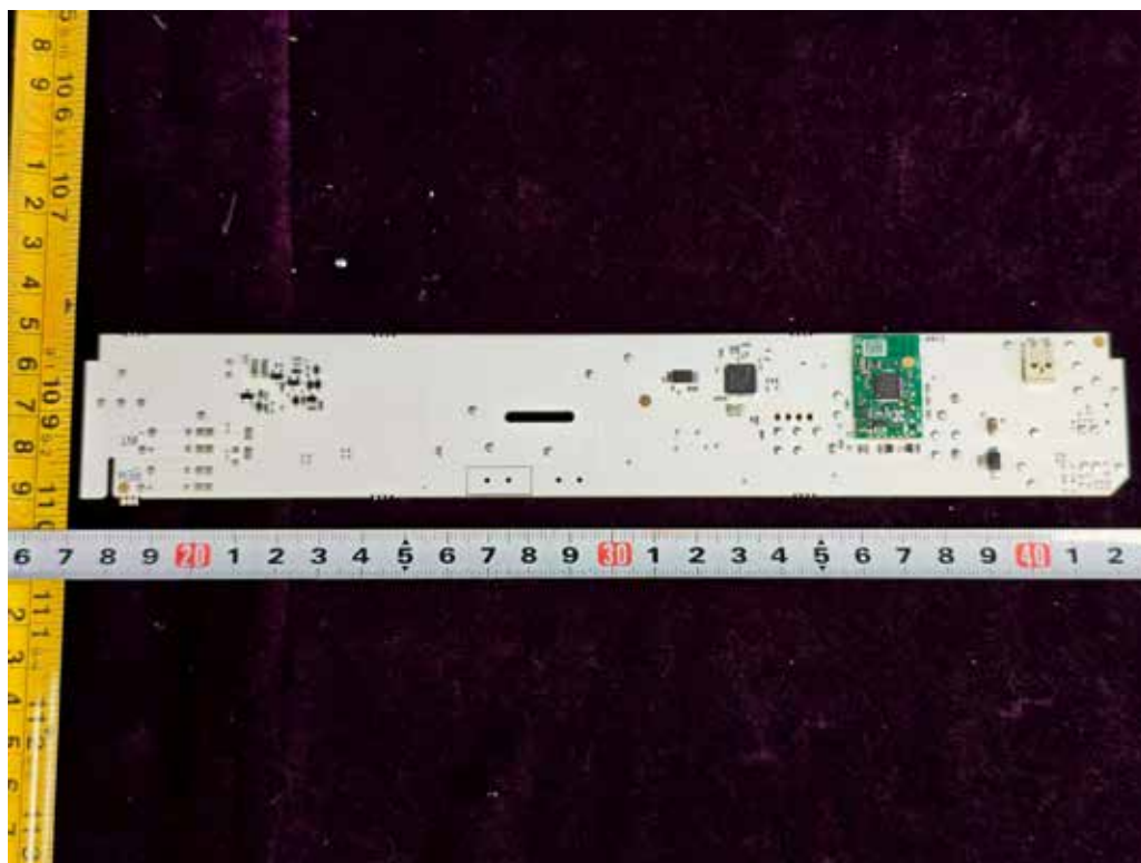
FIGURE 28 EXIT SIGN WITH FIRSTLINK (BXBWFL1) BOARD2-2
