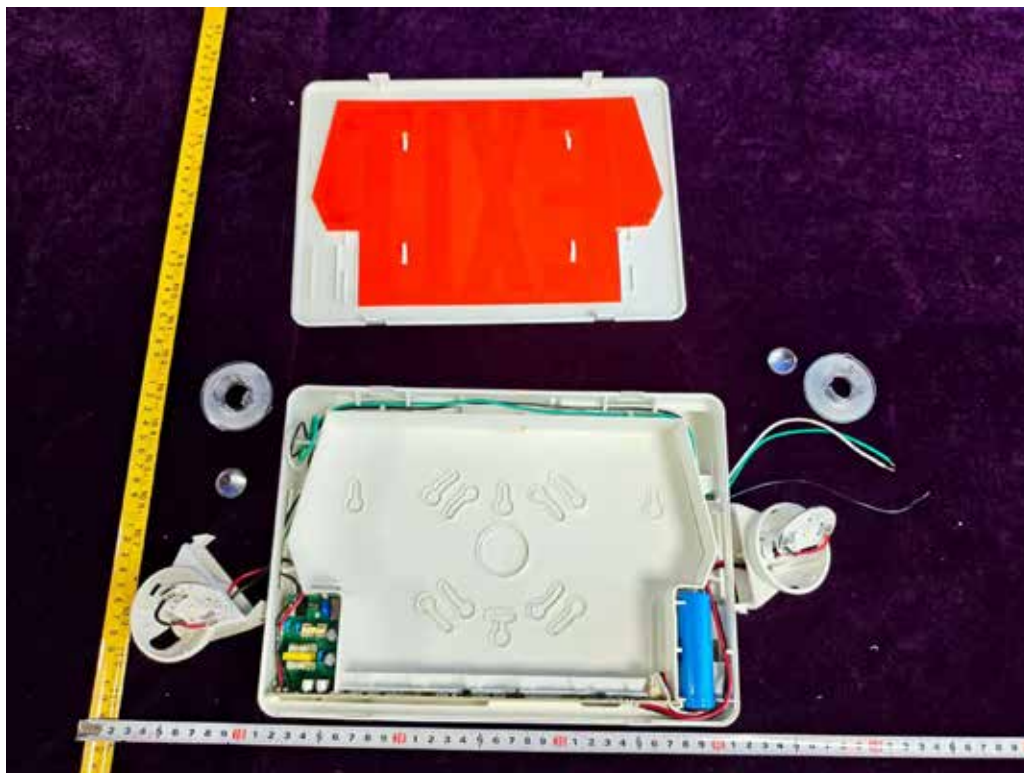
FIGURE 8 COMBO EXIT SIGN WITH FIRSTLINK (BCB4WFL1) BOARD1-1
