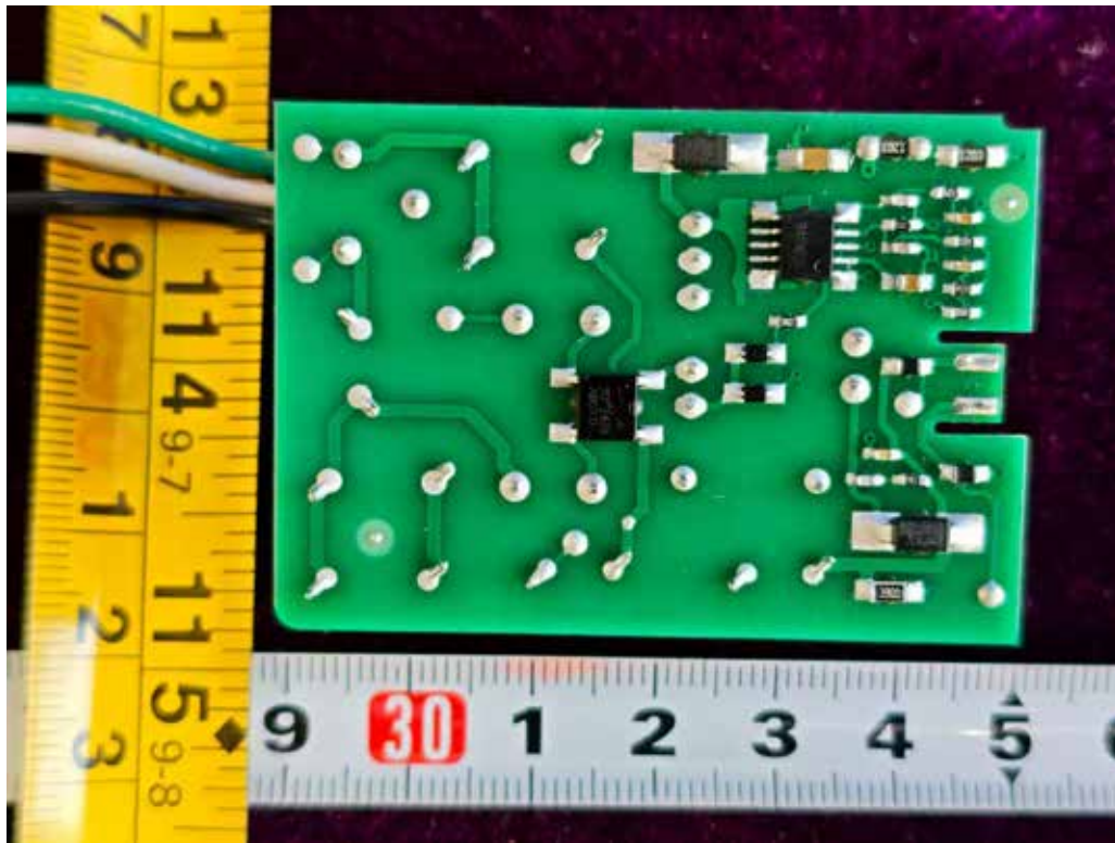
FIGURE 10 COMBO EXIT SIGN WITH FIRSTLINK (BCB4WFL1) BOARD2-1
