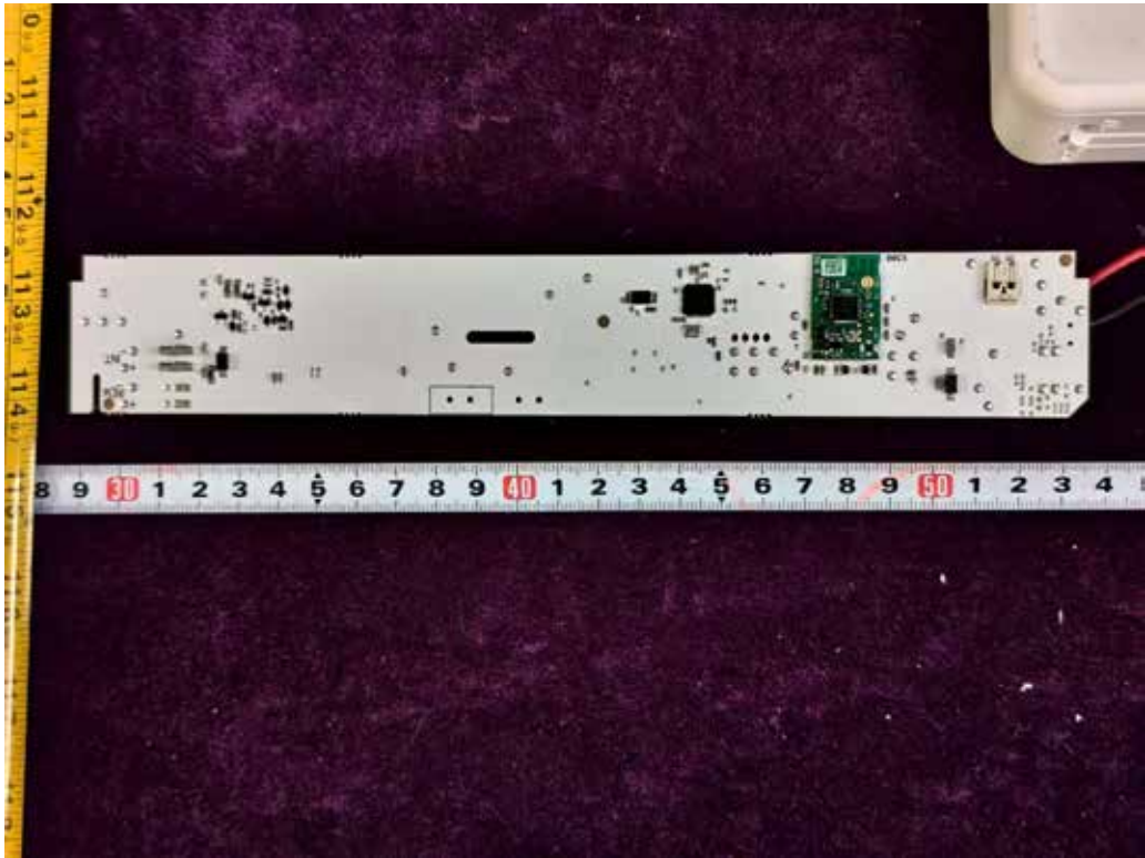
FIGURE 12 COMBO EXIT SIGN WITH FIRSTLINK (BCB4WFL1) BOARD2-3
