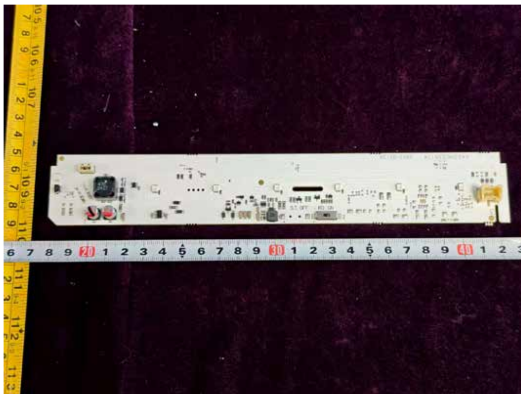
FIGURE 27 EXIT SIGN WITH FIRSTLINK (BXBWFL1) BOARD2-1
