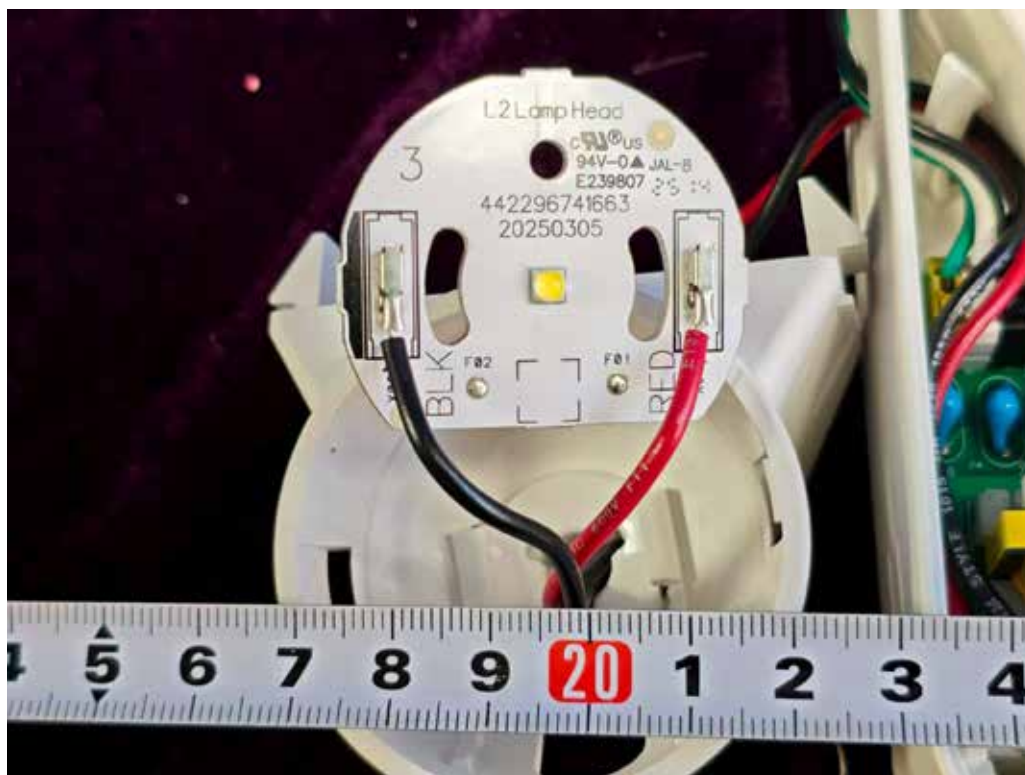
FIGURE 14 COMBO EXIT SIGN WITH FIRSTLINK (BCB4WFL1) BOARD3-2
