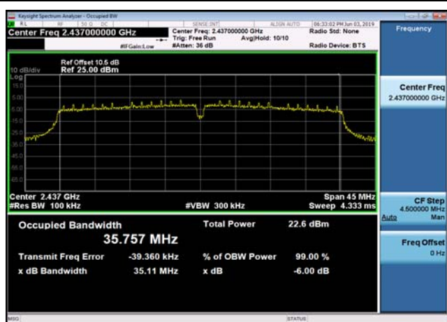
6dB Bandwidth-802.11n(HT40),2437MHz
