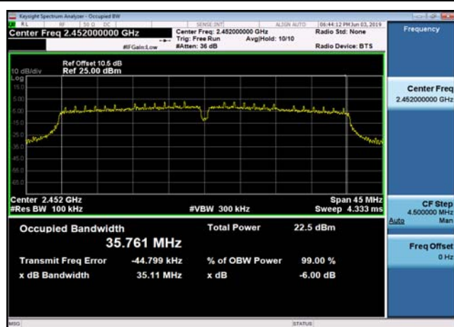
6dB Bandwidth-802.11n(HT40),2452MHz
