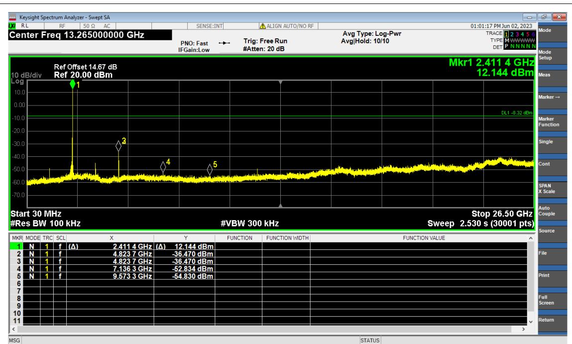
Tx. Spurious NVNT user 2412MHz Ant1 Emission
