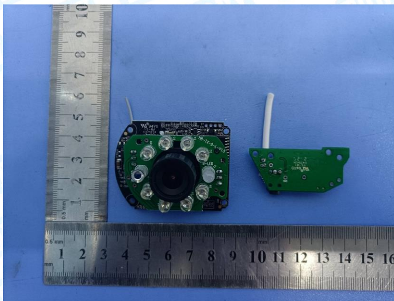
Photo 12 Appearance of PCB
