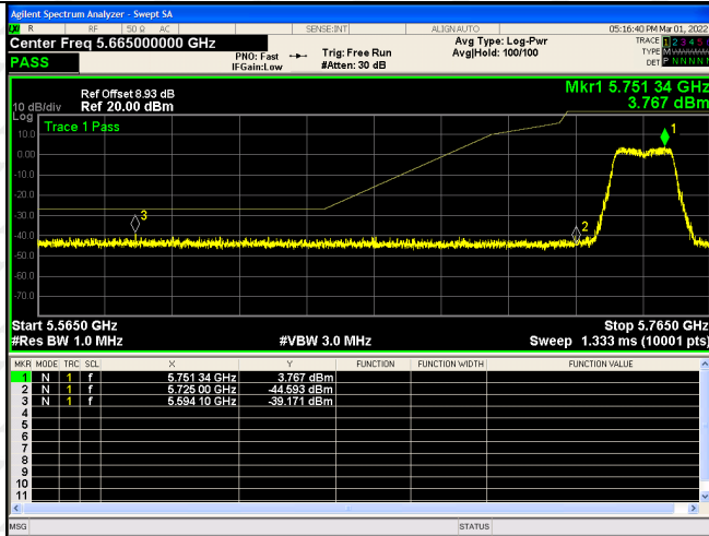
802.11ac(VH40)-5755
