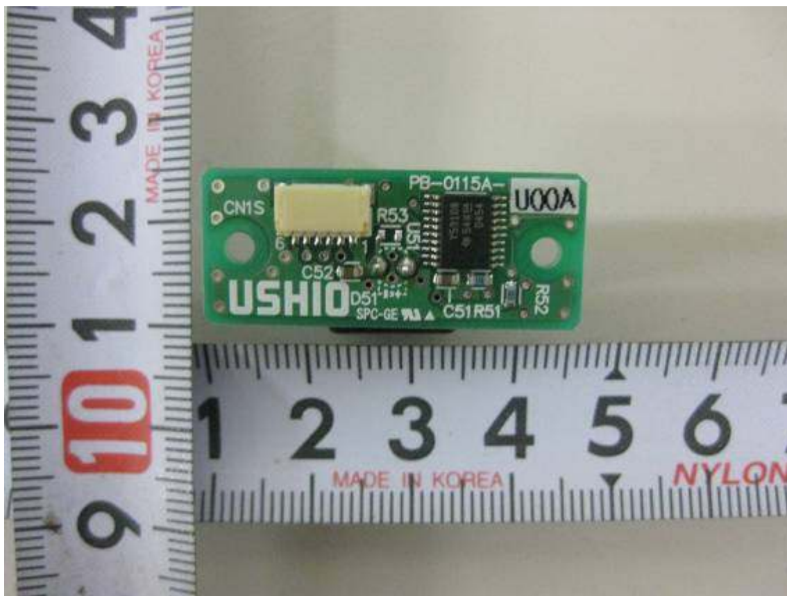
PCB:PB-0115A
