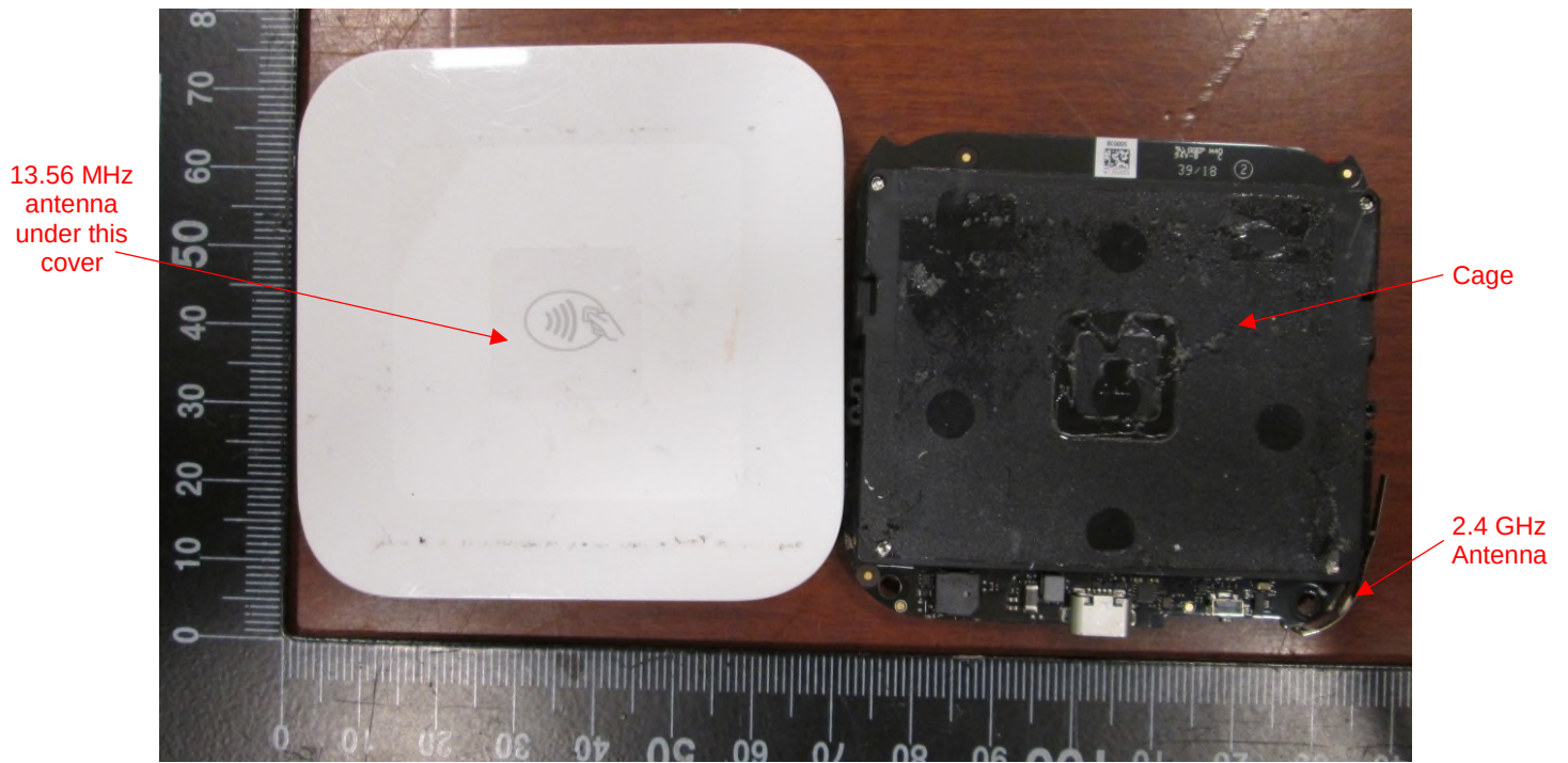
EUT – Internal view 2 PCB removed from enclosure
