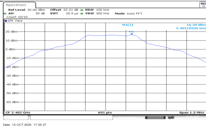
DH5_Ant2_2402_0~Reference
