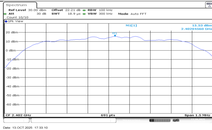
3DH5_Ant2_2402_0~Reference
