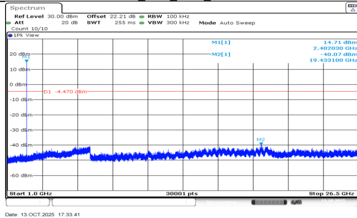
3DH5_Ant2_2402_1000~26500
