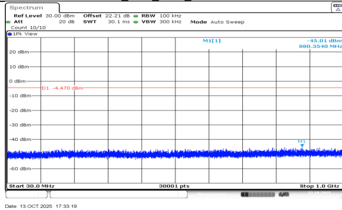
3DH5_Ant2_2402_30~1000
