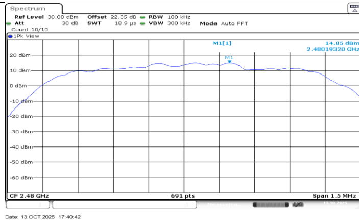
3DH5_Ant2_2480_0~Reference
