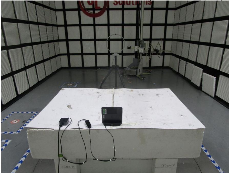
RADIATED SETUP (X axis)
